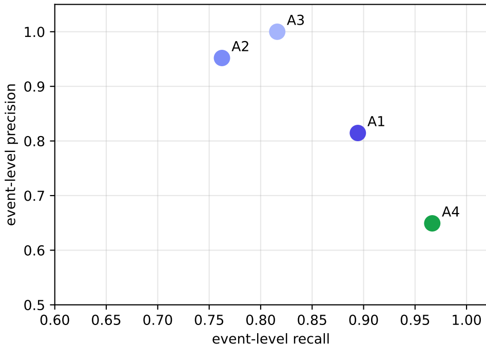
Event-level: LLM arms are more precise than rules (multi-stage)
