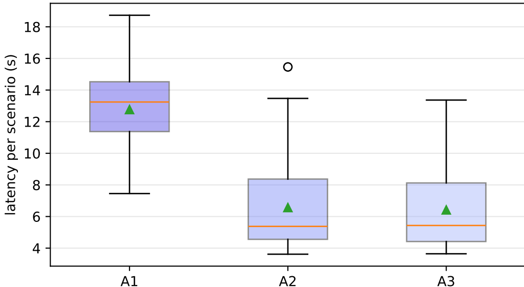
Latency distribution per LLM arm (32B, multi-stage)
