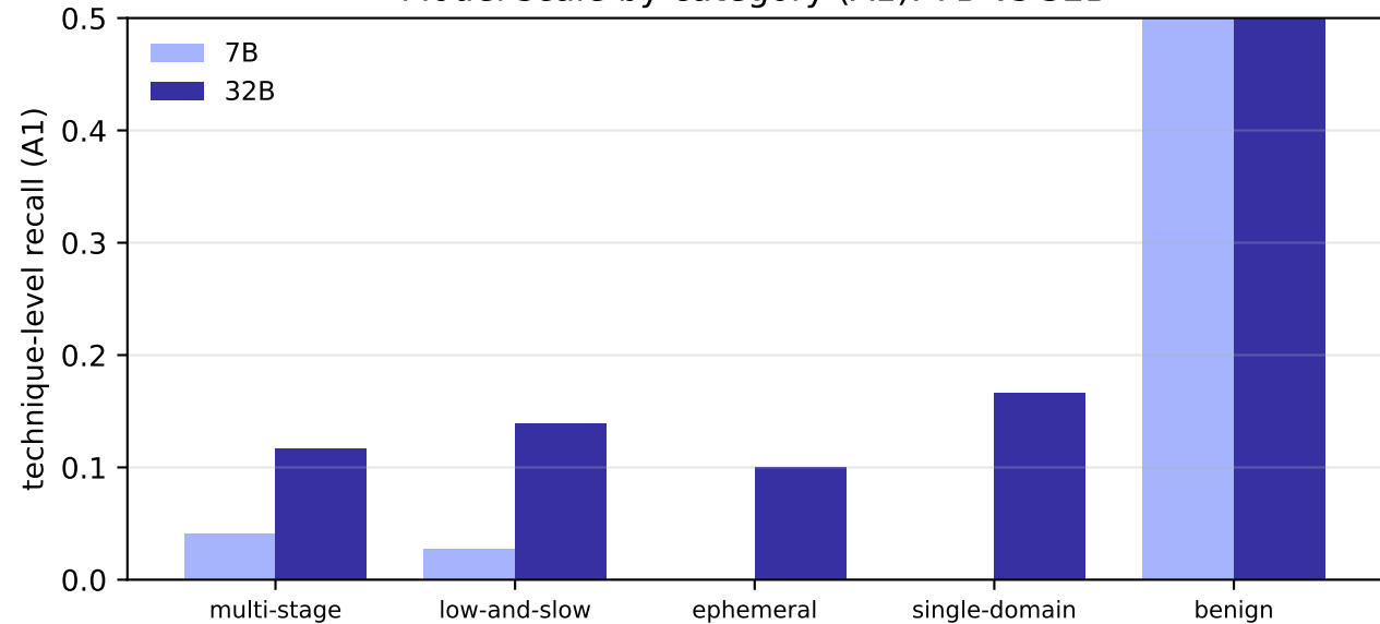
Model scale by category (A1): 7B vs 32B
