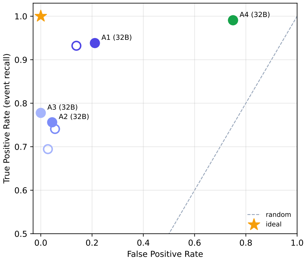
ROC space — arms as operating points (multi-stage) filled = 32B, hollow = 7B
