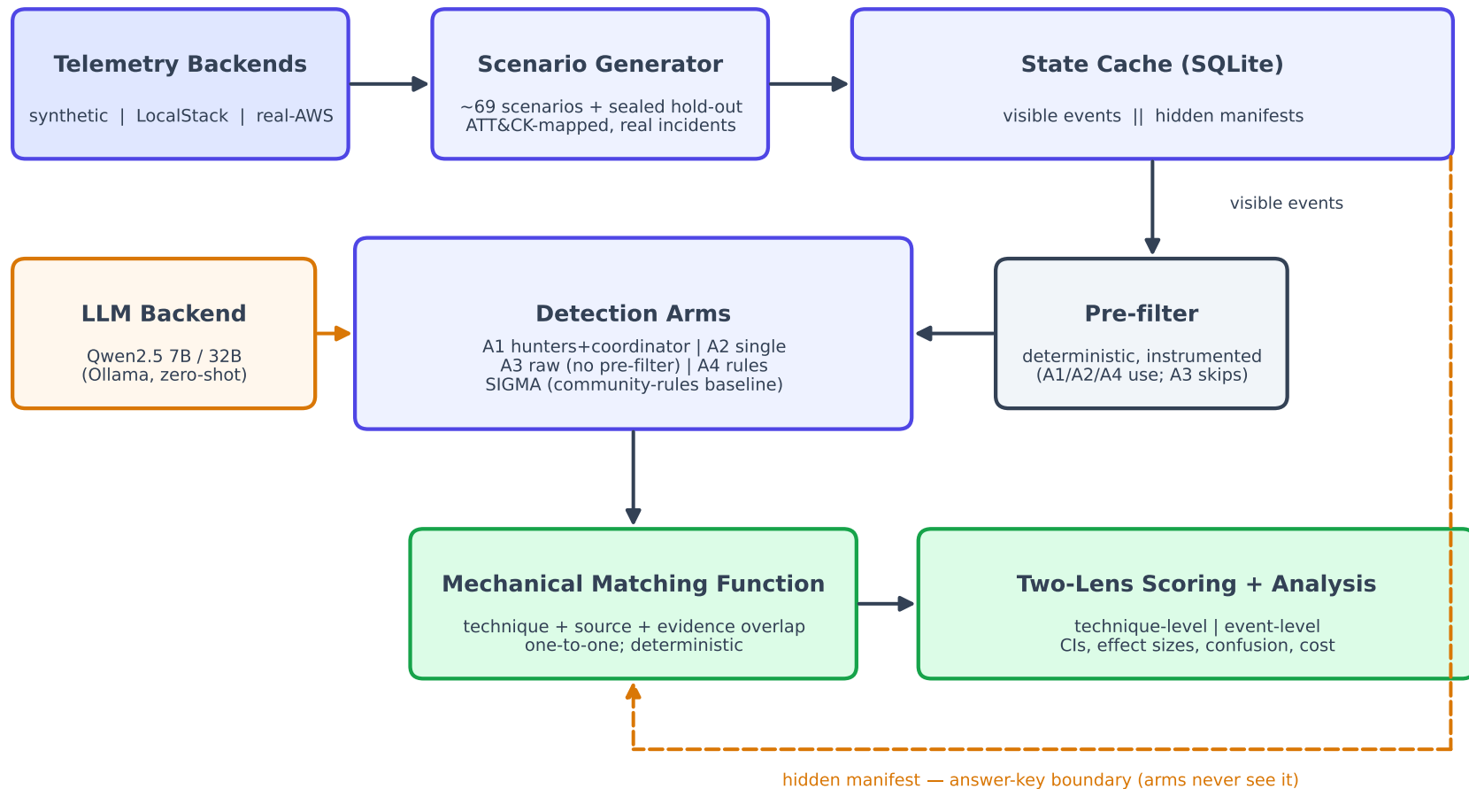
Fig. 1. The CloudKC-Bench framework: data flow from telemetry capture to two-lens scoring.
