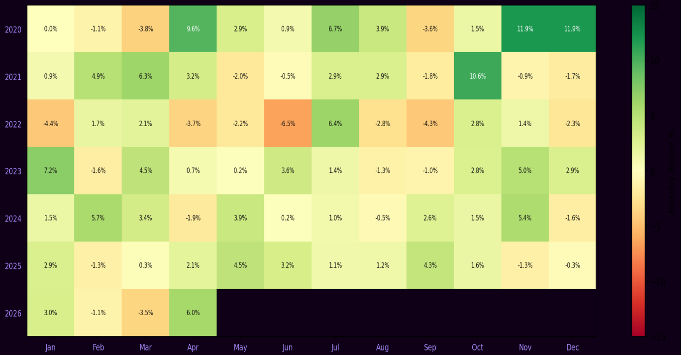
Regime Model — Monthly Returns Heatmap
