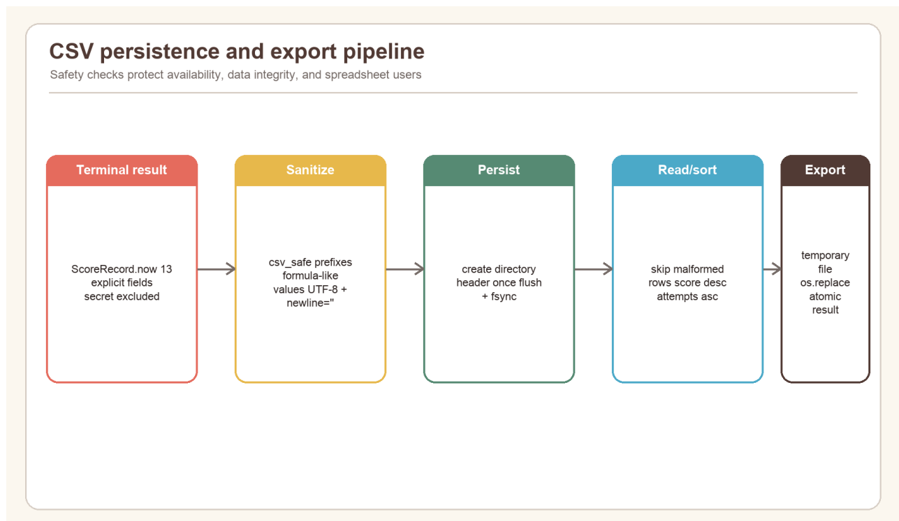
Figure 6. Defensive local persistence and atomic export pipeline.
