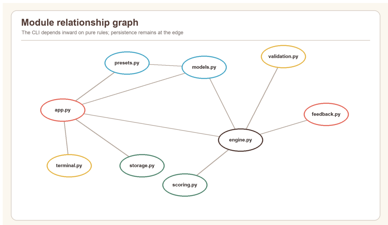
Figure 7. CLI and canonical-core module relationship graph.
