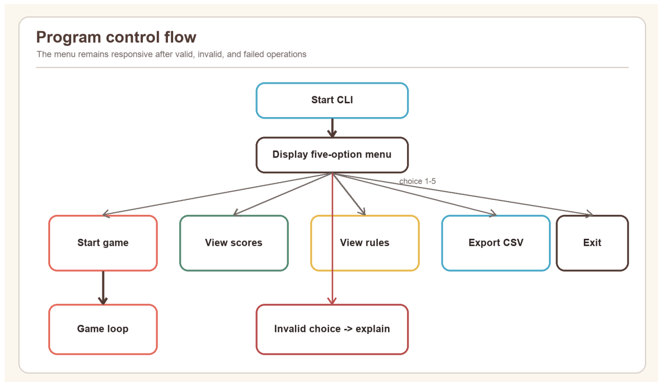
Figure 8. Top-level menu and control-flow design.
