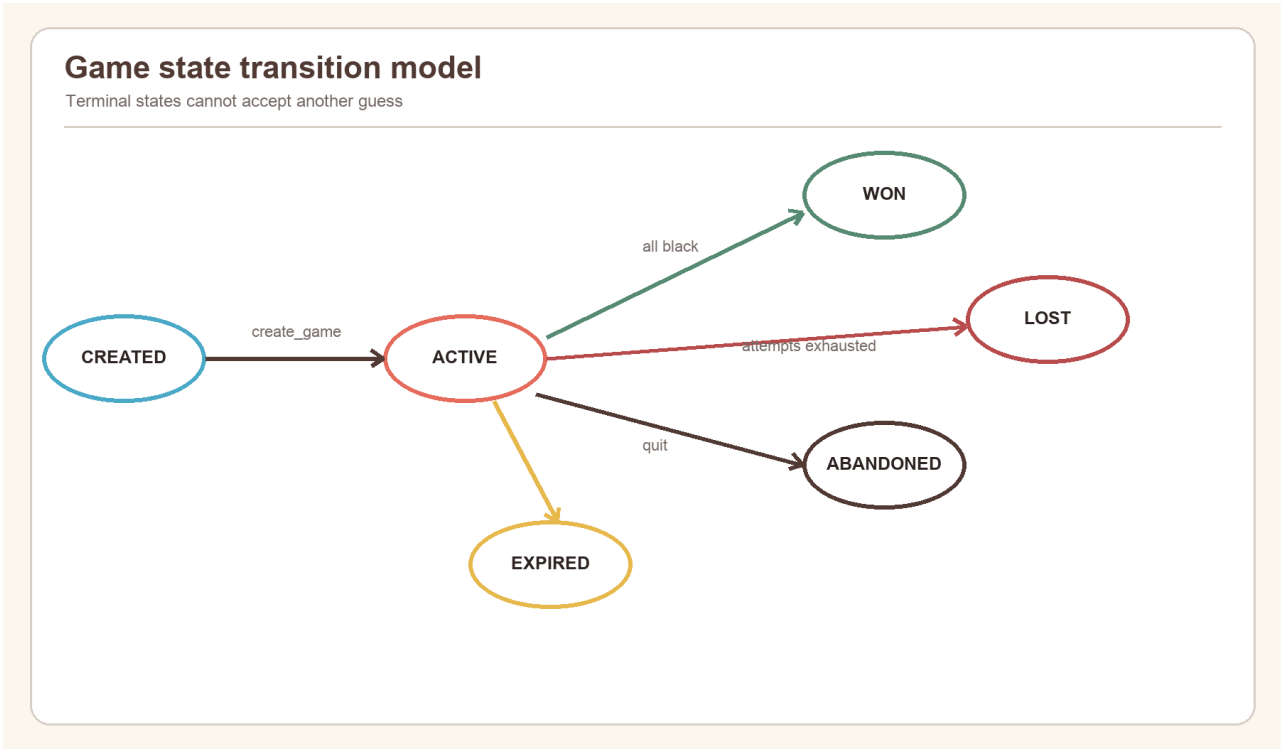
Figure 11. Legal game-state transitions.
