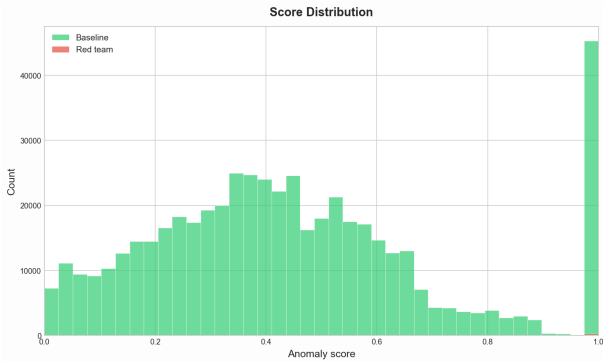
Figure 2: Anomaly score distribution for the combined method. Baseline edges (green) span the full score range with a spike at 1.0 from path boosting. Red-team edges (orange) are concentrated at high scores but are too few to be visible in the histogram. (Figure by: Ibrahim Pehlivan)
