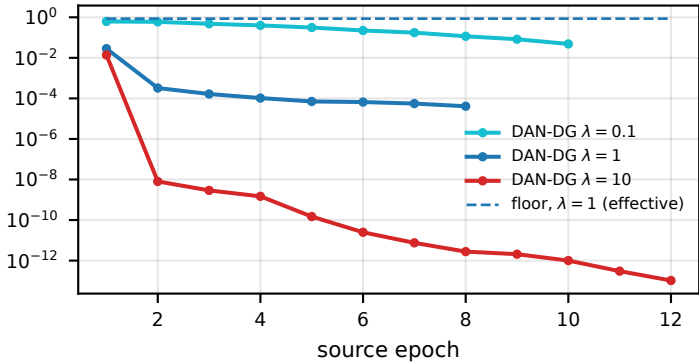
Epoch-mean batch median sq. distance (MMD bandwidth scale)
