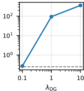
Sharpness proxy \Delta_{\text{sharp}}
