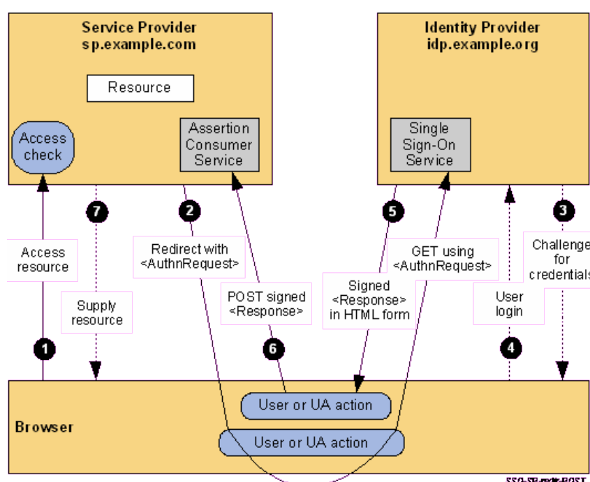
Figure 2.1: SP-Initiated SSO with Redirect and POST Bindings [SAMLOverview]
