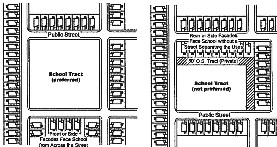
Figure 1: Neighborhood Layouts Adjacent to School (not to scale)
