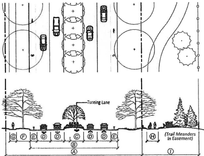
Figure 3: Urban Arterial Street Section
