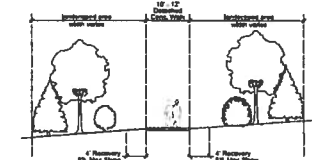
Typical Cheyenne Greenway Trail scale: NTS
