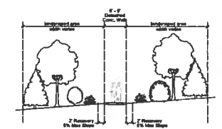
Typical Sweetgrass Low Impact Trail scale: NTS
