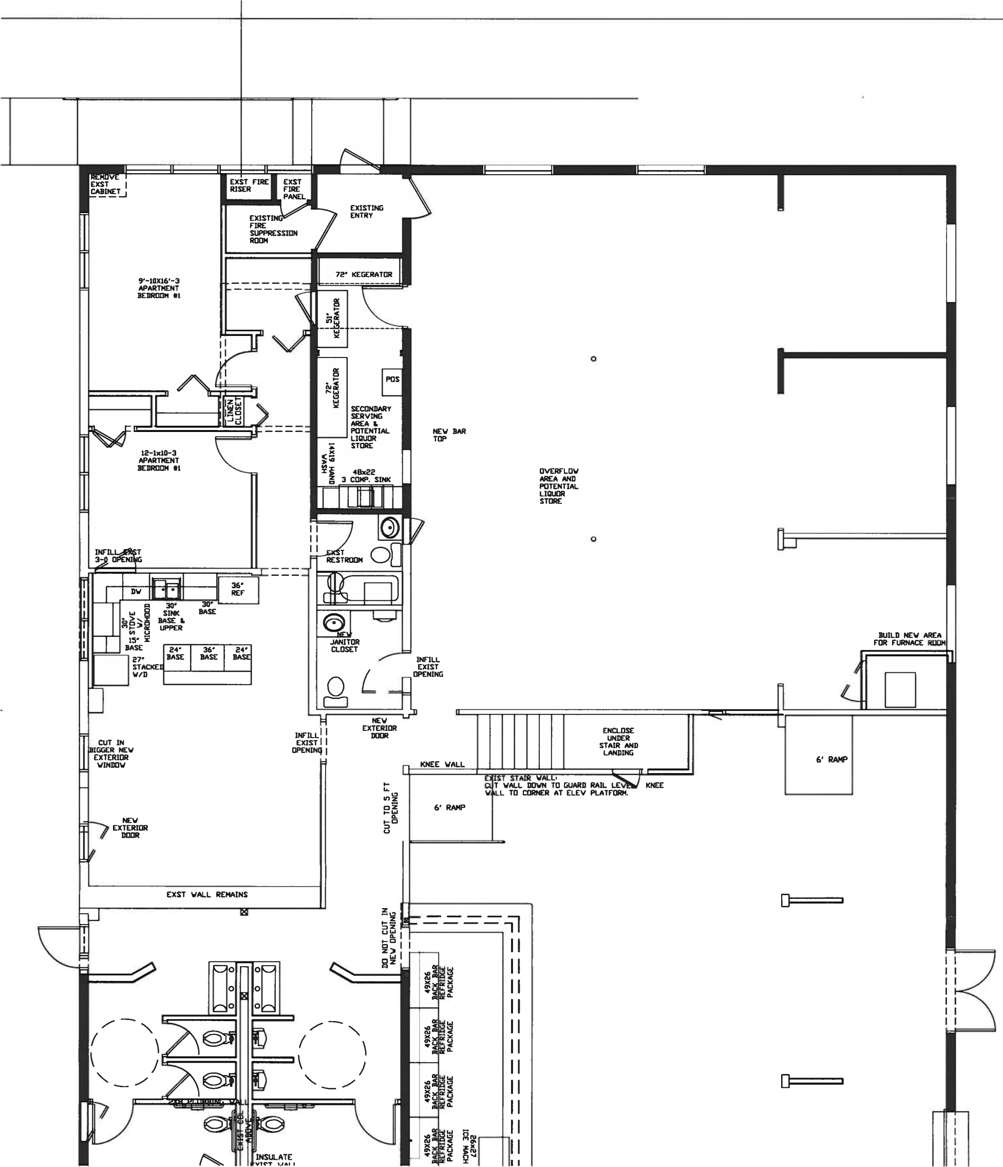
WESTBY EDGE WAREHOUSE - OVERFLOW/PACKAGE AREA FLOOR PLAN 714 W. 20TH STREET CHEYENNE, LARAMIE COUNTY, WY
