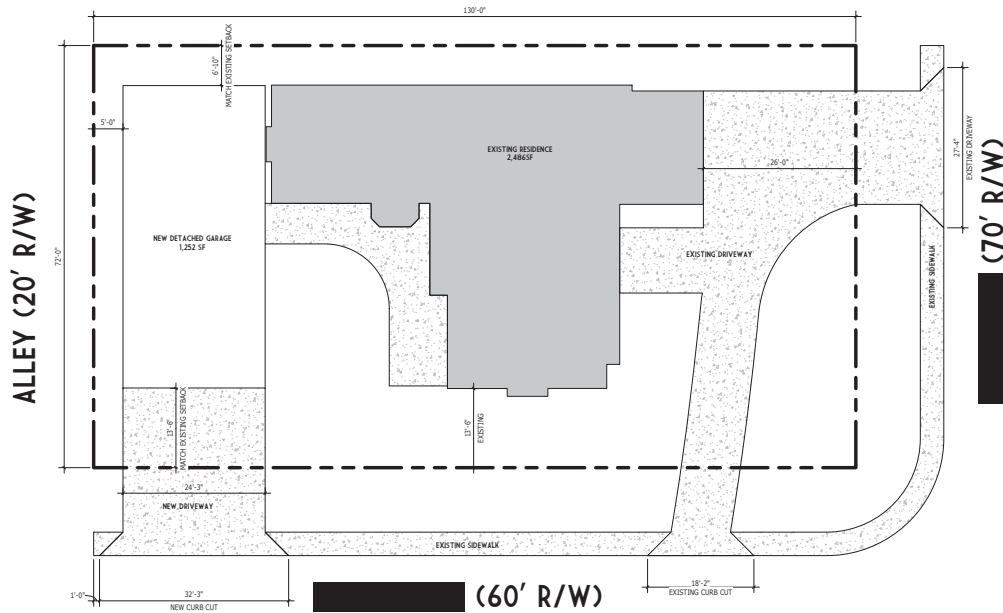
1 SITE PLAN 1" = 10'-0"
