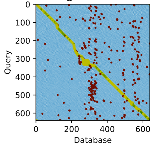
R@1 = 0.3250
