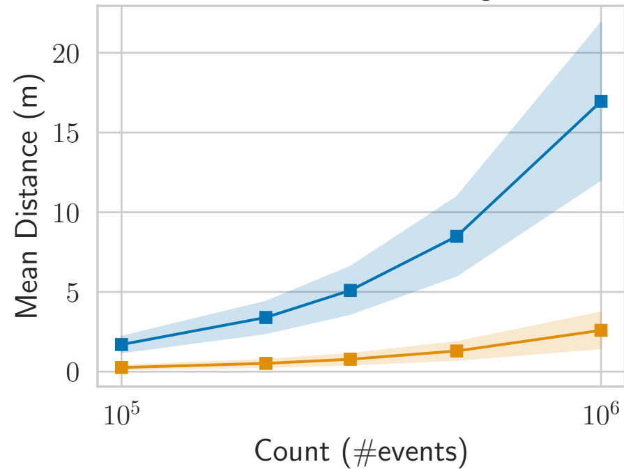
Count-based Binning
