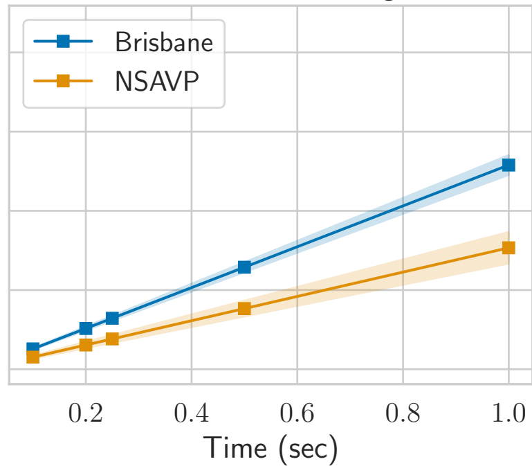
Time-based Binning
