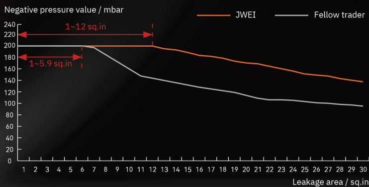
JWEI Cutting Machine Negative Pressure Curve Chart
