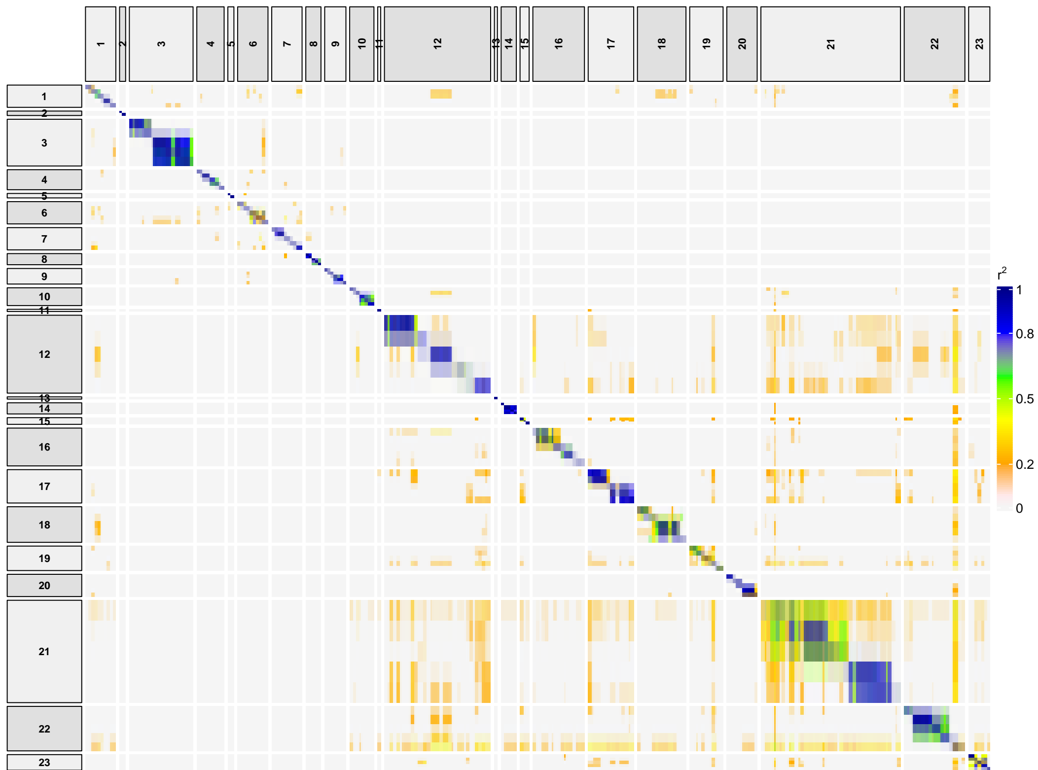
Genome-Wide Linkage Disequilibrium of High-Loading SNPs
