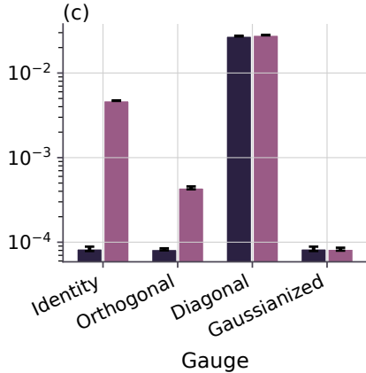
Projected Gaussianity score
