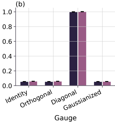
Embedding covariance anisotropy
