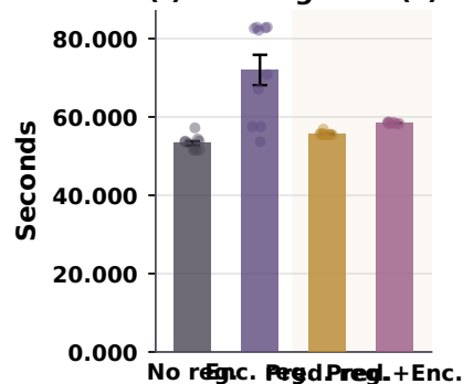
(f) Training time (s)
