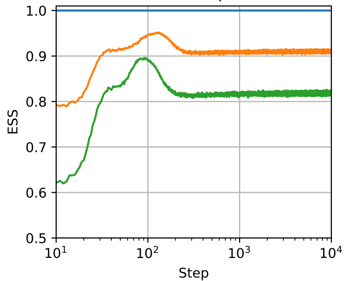
Effective Sample Size
