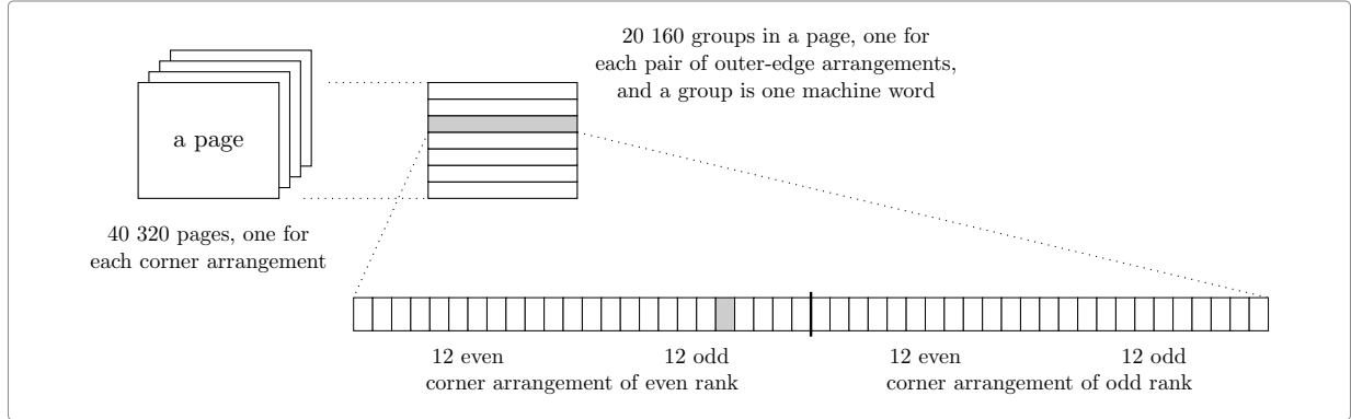
Figure 9: The map, from the outside in. A page for each arrangement of the corners, a group in the page for each pair of outer-edge arrangements, and a bit in the group for each arrangement of the 4 middle edges, the 12 even ones low and the 12 odd ones high. One word holds the same group on the 2 pages of a pair.
