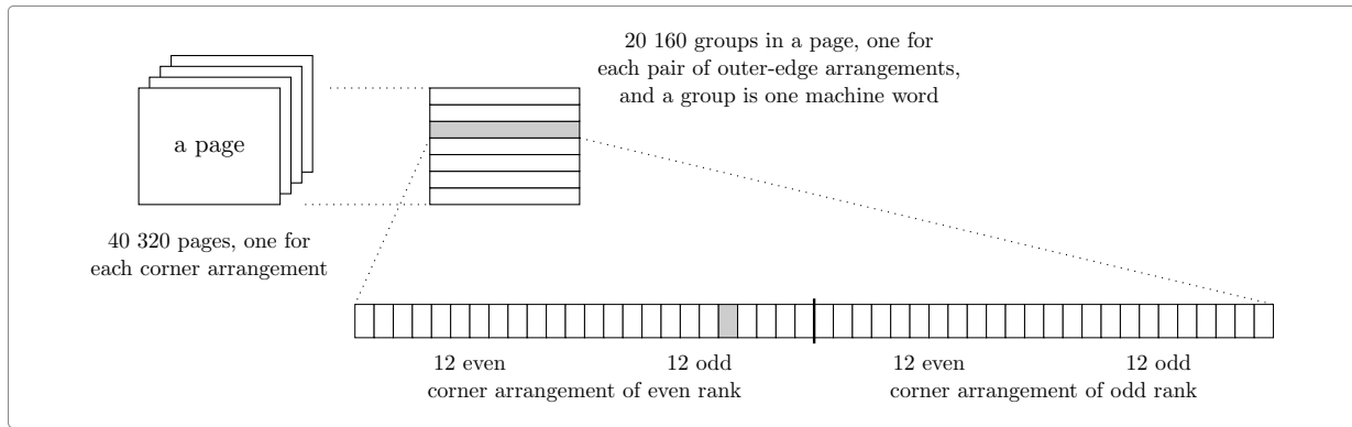
Figure 13: The map: a page per corner arrangement, a group for each pair of outer-edge arrangements and a bit for each arrangement of the 4 middle edges, the 12 even ones low and the 12 odd ones high.
