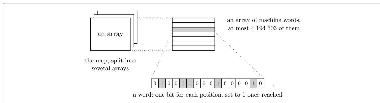
Figure 12: The map of a coset. One bit for each position of the coset, the bits kept in machine words and the words in arrays, as many arrays as Rocq's limit on the length of an array asks for.
