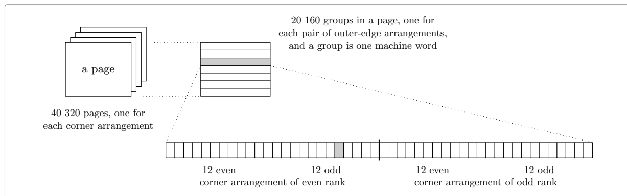
Figure 10: The map, from the outside in. A page for each arrangement of the corners, a group in the page for each pair of outer-edge arrangements and a bit in the group for each arrangement of the 4 middle edges, the 12 even ones low and the 12 odd ones high. One word holds the same group on the 2 pages of a pair.
