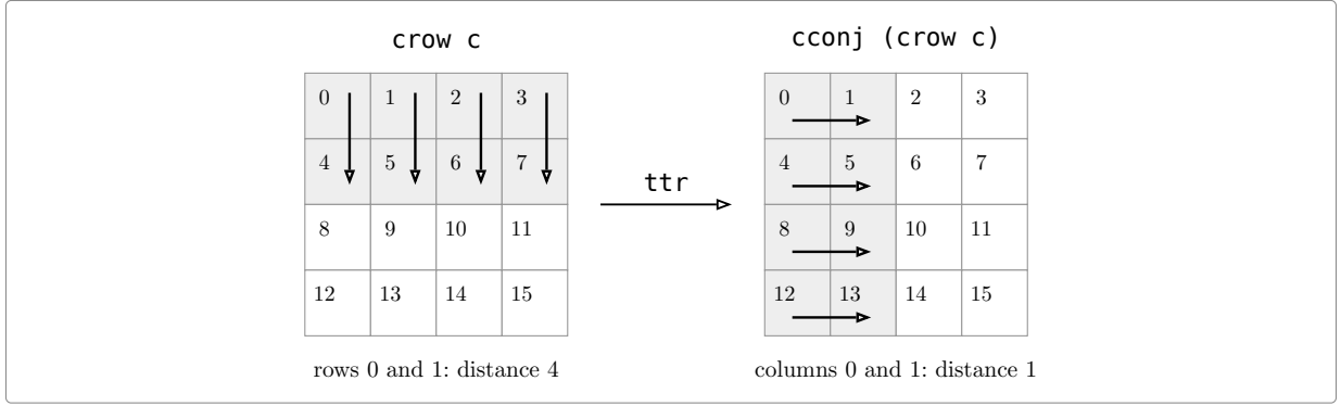
Figure 3: crow and cconj on a 4 \times 4 square, for c the single comparison cswap 0 1 on four places. The sixteen places are numbered across the rows, so place i sits at row i/4 and column i \bmod 4 . crow c applies c to the row number: it compares row 0 with row 1, place by place, which on the flat array is four comparisons at distance four. Reading it through the transpose gives the same comparisons on the columns, at distance one, which is what one vector instruction does. An arrow points at the place that receives the larger value.
