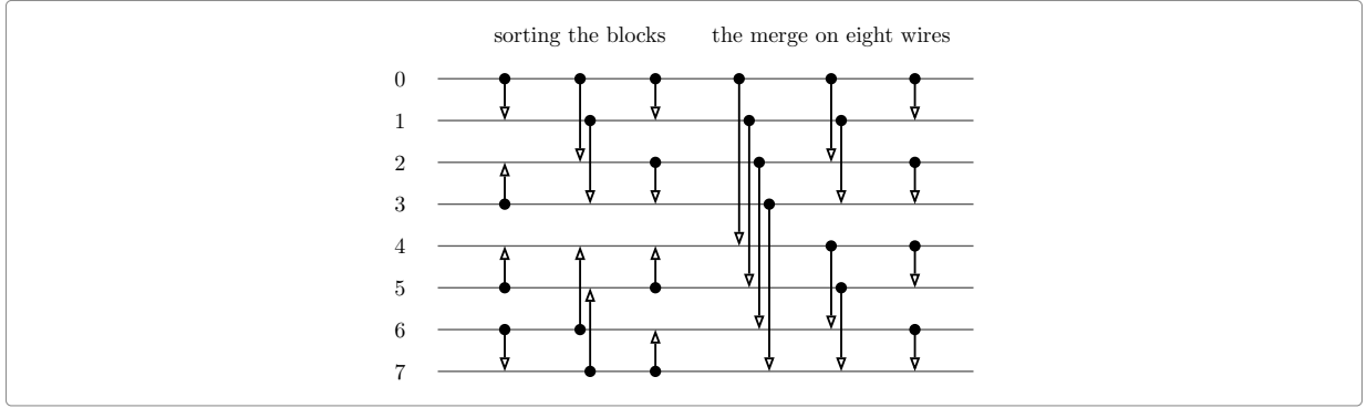
Figure 5: bfsort false 3 , the bitonic sorter on eight wires. An arrow points at the end that receives the larger value. The first three columns are the two halves being sorted, the first one upwards and the second downwards; inside each of them the same rule is applied again. The last three columns are the merge of Figure 4. Turn the arrows of those last three columns round, and the sorter runs downwards.
