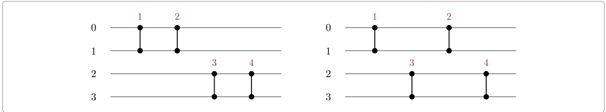
Figure 10: The colour of a comparison is the half of the array where it sits. The left list does the top half first. The right list takes the two halves alternately. Different colours never share a place, and each colour appears in the same order in both lists (1 then 2, and 3 then 4). So the two lists compute the same thing.
