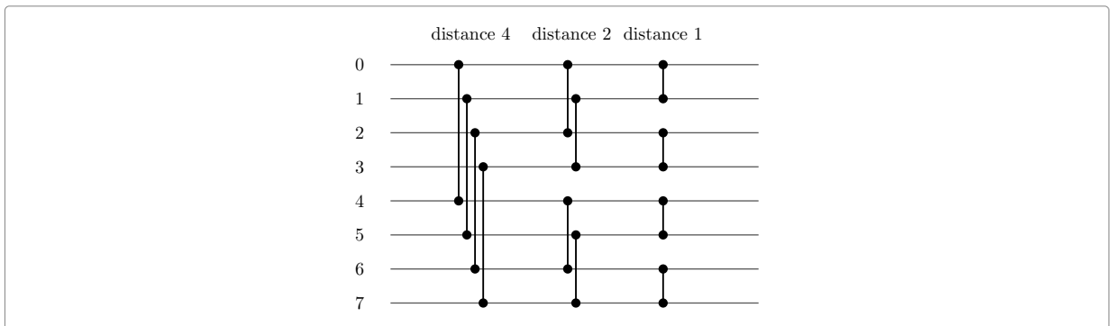
Figure 4: Sorting a bitonic sequence of eight values: one half-cleaner at distance four, then one in each half at distance two, then one in each quarter. After the first column, nothing crosses the middle again.
