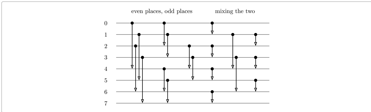
Figure 6: knuth_exchange 3 , the merge exchange on eight wires, six stages and nineteen comparisons. The first three columns sort the four even places and the four odd places, by the same network read twice. The fourth column compares each pair of neighbours, and the last two are the jumps, at distance three and then at distance one. Every comparison sends the smaller value upwards, so no direction is needed anywhere.
