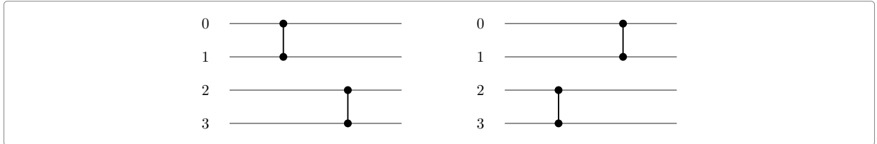
Figure 9: The same two comparisons in the two possible orders. They touch four different places, so nothing can change: whichever is done first, the result is the same.
