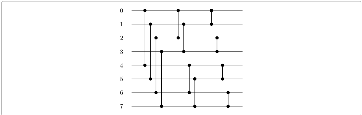
Figure 11: The table N_mrg8 : twelve comparisons between eight registers. It is the bitonic merge on eight wires, one distance at a time. Each wire here is q consecutive places of the array, so each comparison drawn is q comparisons of the array, and the three columns are the levels at 4q , at 2q and at q .
