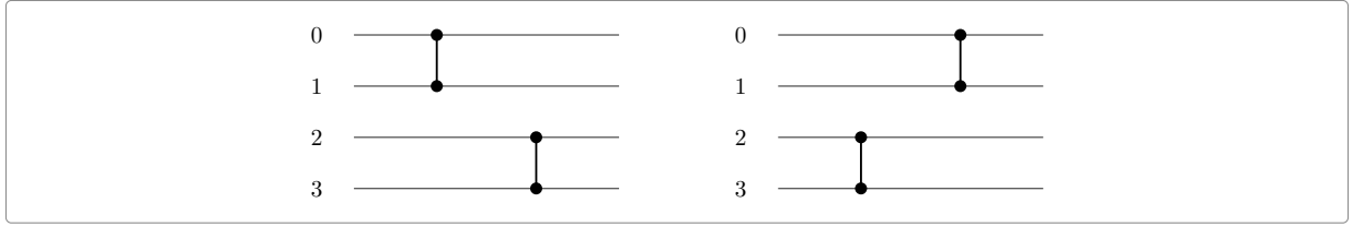
Figure 8: The same two comparisons in the two possible orders. They touch four different places, so nothing can change: whichever is done first, the result is the same.
