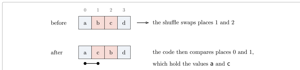
Figure 7: A shuffle changes the meaning of a place. The comparison that the code writes as (0, 1) is, in terms of values, the pair (a, c) .
