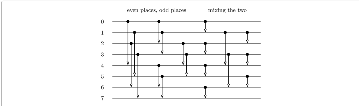
Figure 5: knuth_exchange 3 , the merge exchange on eight wires, six stages and nineteen comparisons. The first three columns sort the four even places and the four odd places, by the same network read twice. The fourth column compares each pair of neighbours, and the last two are the jumps, at distance three and then at distance one. Every comparison sends the smaller value upwards, so no direction is needed anywhere.
