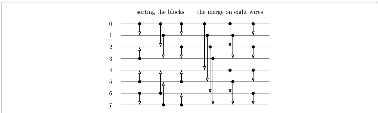
Figure 4: bfsort false 3 , the bitonic sorter on eight wires. An arrow points at the end that receives the larger value. The first three columns are the two halves being sorted, the first one upwards and the second downwards; inside each of them the same rule is applied again. The last three columns are the merge of Figure 3. Turn the arrows of those last three columns round, and the sorter runs downwards.
