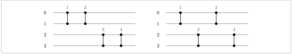
Figure 9: The colour of a comparison is the half of the array where it sits. The left list does the top half first. The right list takes the two halves alternately. Different colours never share a place, and each colour appears in the same order in both lists (1 then 2, and 3 then 4). So the two lists compute the same thing.
