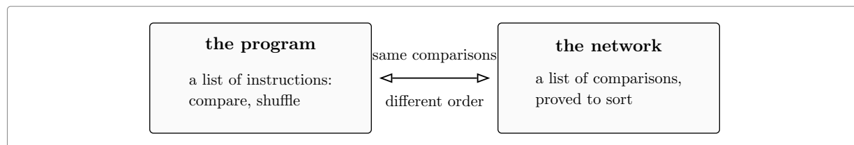
Figure 6: The two sides and the bridge between them. The left box is what the machine runs. The right box is what we can reason about. The bridge says that they perform the same comparisons.
