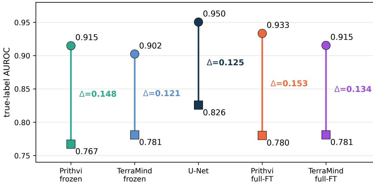
Transfer gap: in-region (•) vs all-30 cross-region (■)
