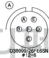
D38999/26FE6SN #12-6
