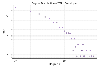
(a) Degree distribution (log-log).
