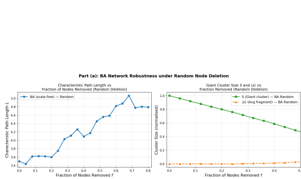
(a) L(f) and S(f) under random deletion on the BA network.
