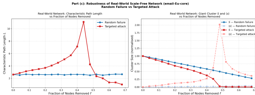
Figure 6: S and \langle s \rangle on email-Eu-core under random failure and targeted attack.
