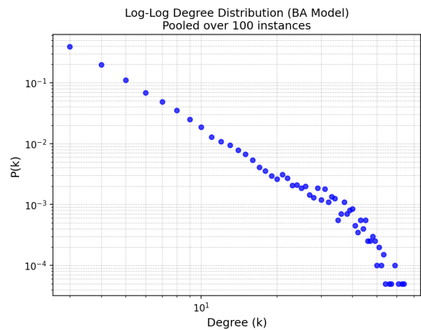
(b) Log-log degree distribution pooled over 100 instances.
