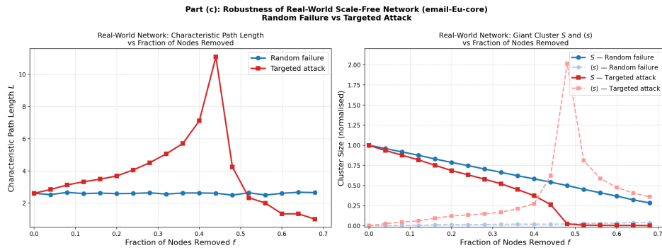
Figure 5: S and \langle s \rangle on email-Eu-core under random failure and targeted attack.
