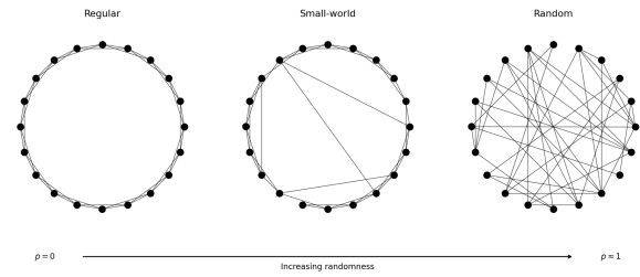
(b) Network structure at p = 0 , p = 0.1 , p = 1 .
