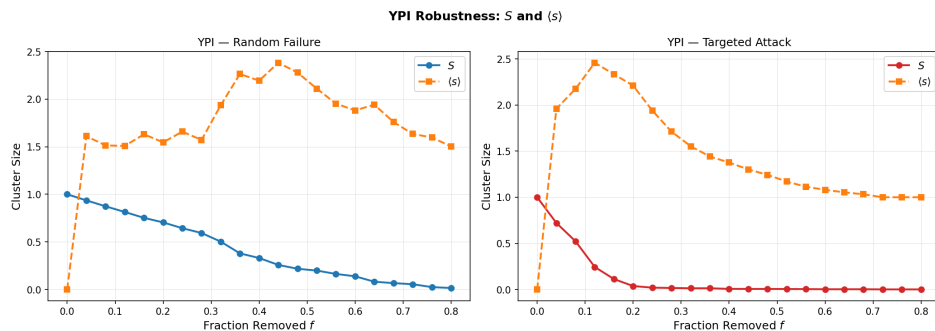
Figure 8: S and \langle s \rangle under random failure and targeted attack on YPI.
