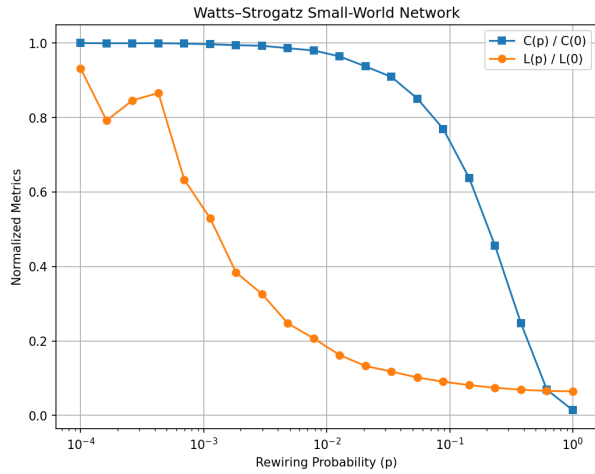
(a) Scaled C(p)/C(0) and L(p)/L(0) vs rewiring probability.
