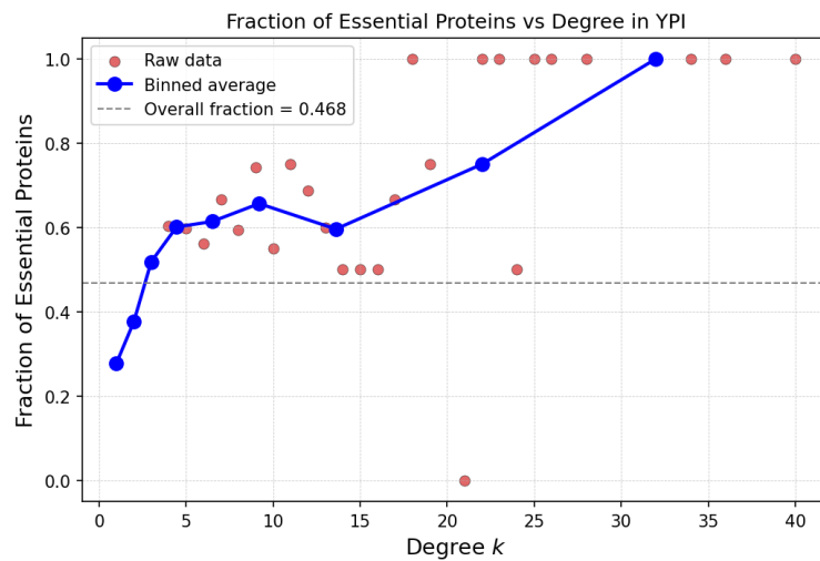
Figure 7: Fraction of essential proteins vs degree k . The trend is clear above k \approx 5 .
