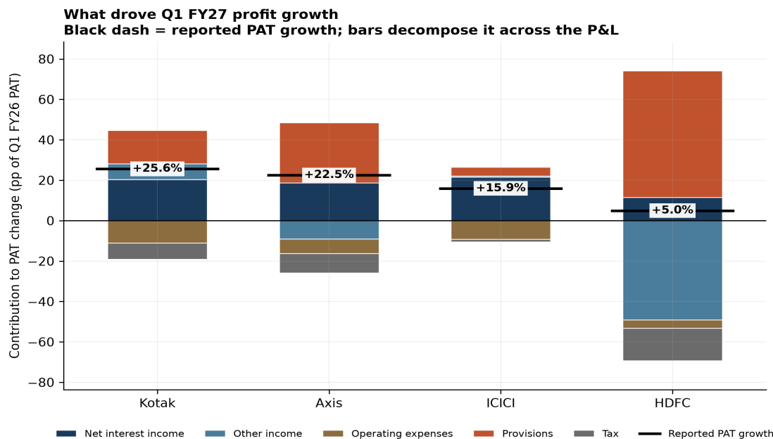
Figure 1. The same decomposition. Bars stack above and below zero by sign; the black dash is each bank's reported PAT growth.
