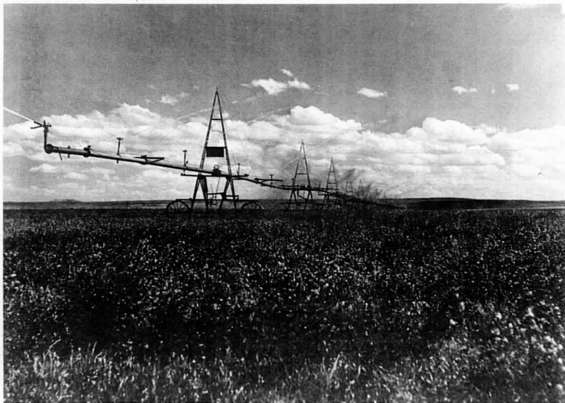
GIANT SELF-PROPELLED IRRIGATION SYSTEM AT WORK --This is the type of apparatus used to water alfalfa field at View Point Ranch. It takes four days for the line to turn a complete circle. At the end of this time, 160 acres will have been irrigated. The entire watering system irrigates 700 acres every four days. The five wells at the View Point Ranch produce 1,452,672,000 gallons of water a year for the big spread.
