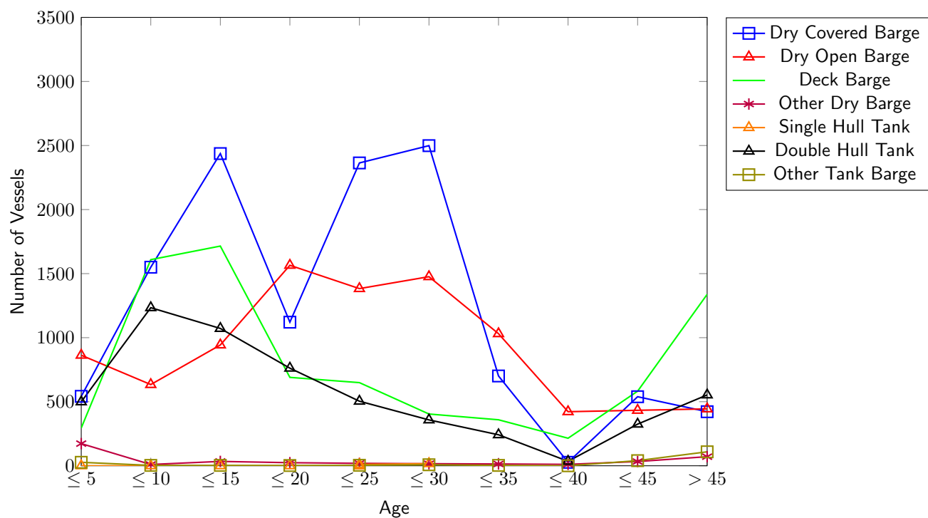
Figure 10: Non Self-Propelled Vessels by Type and Age
