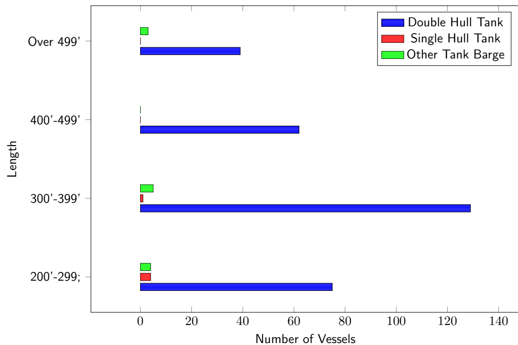
Figure 14: Deep Draft Tank Barge Fleet by Type and Size for 2023
