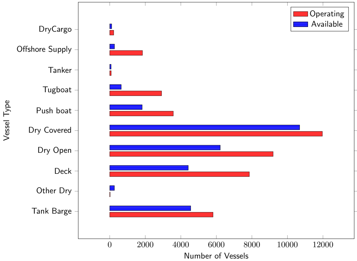
Figure 28: U.S. Flagged Vessels Available Vs. Operating for 2023
