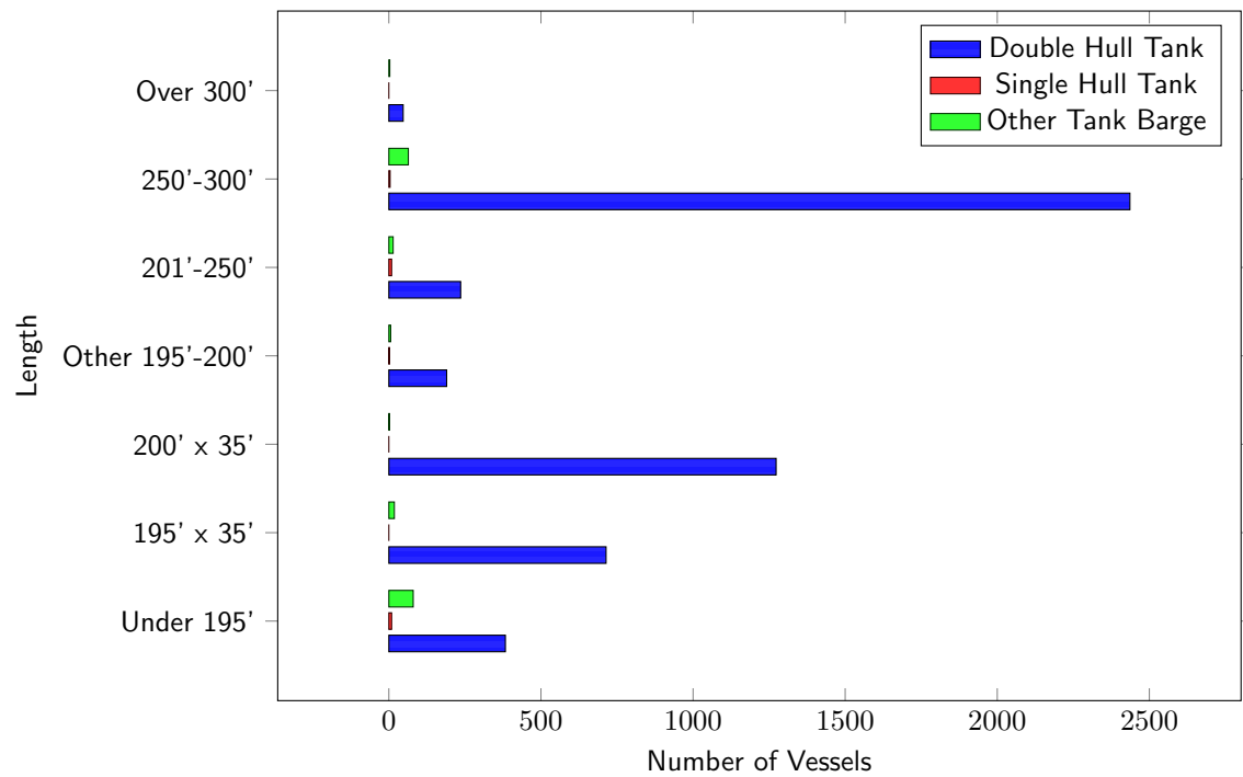
Figure 13: Shallow Draft Tank Barge Fleet by Type and Size for 2023
