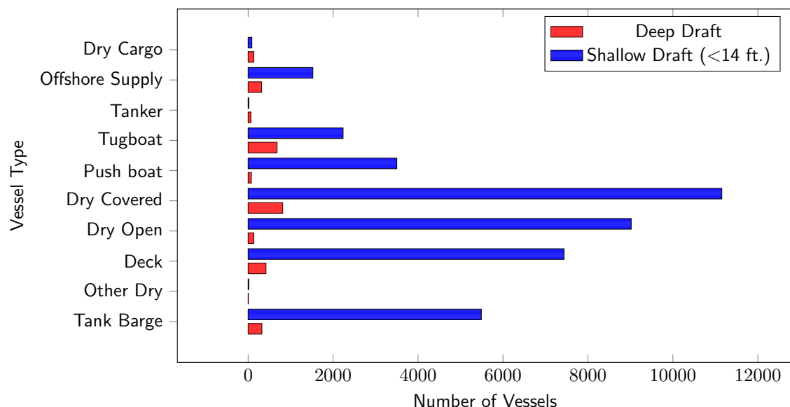
Figure 27: Shallow and Deep Draft Vessels by Vessel Type and Size for 2023
