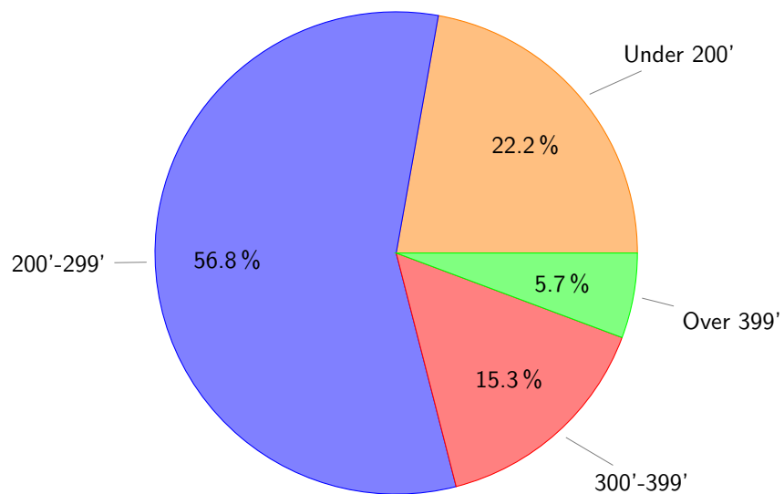
Figure 24: Deep Draft Dry Open Barges by Size
