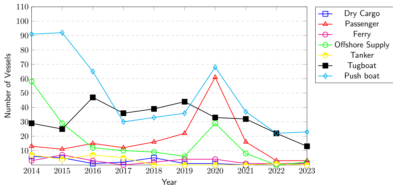
Figure 6: New Construction of Self-Propelled by Vessel Type per Year
