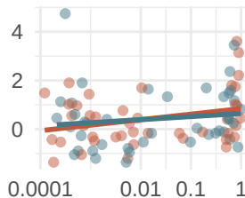
Leaf number
