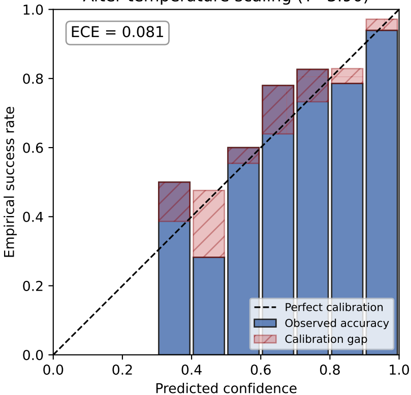
After temperature scaling ( T=3.90 )
