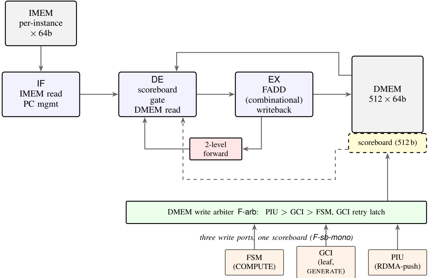
Fig. 11. PE microarchitecture. The three-stage IF–DE–EX pipeline is scoreboard-gated at DE; the scoreboard is a single source of truth for “data present at address a ” across the three agents that write DMEM (PIU, GCI, FSM COMPUTE writeback). A GENERATE is committed by the GCI port, not by a fourth agent. A two-level write-to-read forwarding network (red) handles the BRAM read-first race for back-to-back writes and across-one-stall writes. The DMEM write arbiter (green) enforces the strict-priority PIU > GCI > FSM discipline of F-arb; the GCI retry latch re-asserts the pending write until accepted. No write is silently dropped.
