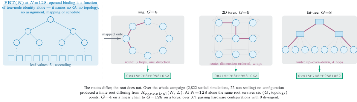
Fig. 6. Claim 1. The same reduction DAG mapped onto different topologies yields the identical 64-bit root: routes differ, the root does not.
