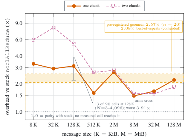
Fig. 22. Measured overhead of the pinned-FBT export against stock ncclAllReduce . Pre-registered and unfavourable; the point estimate is provisional, measured under GPU contention.
