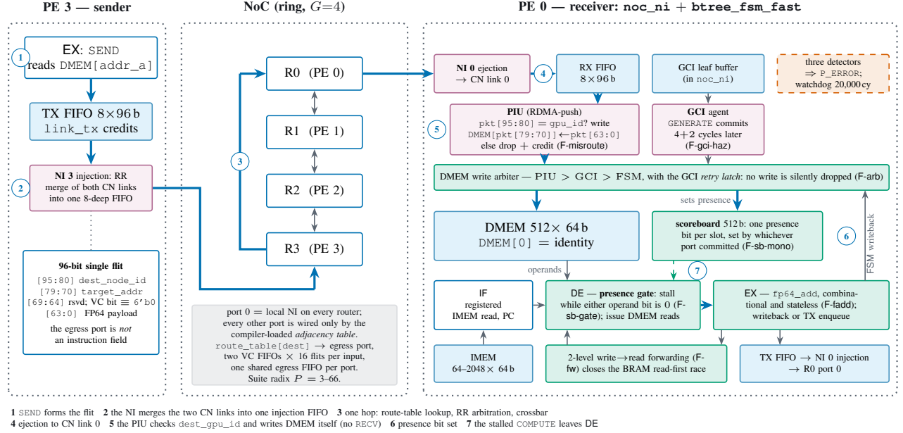
Fig. 10. The fabric: PE, DMEM, scoreboard and the NoC router the packet crosses.
