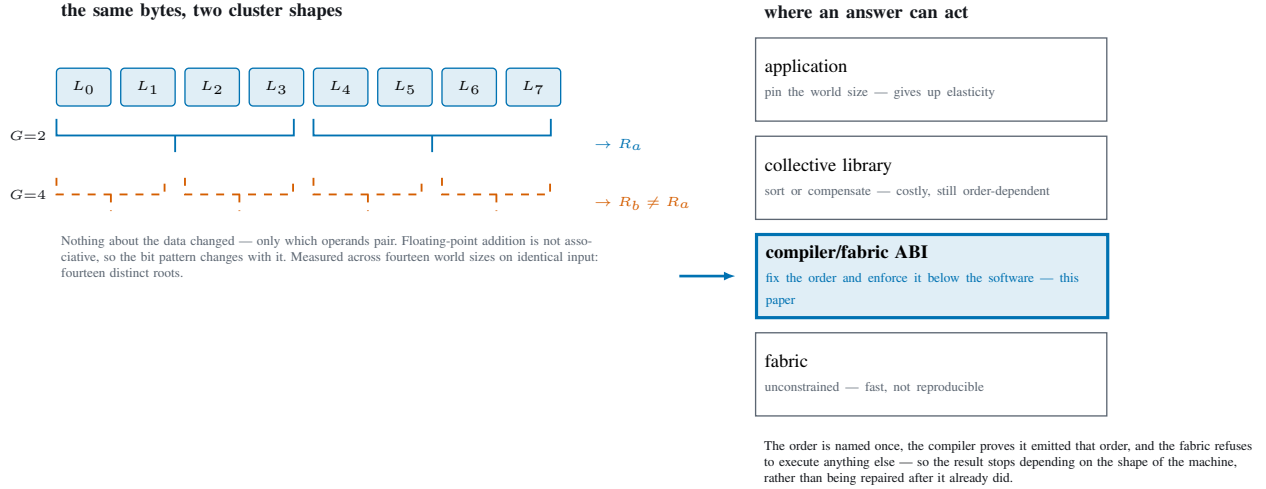
Fig. 1. What cluster reshape does to a reduction, and where an answer can act. Only the grouping changes; because floating-point addition is not associative, the bit pattern changes with it. Existing answers act above the fabric and pay for it in elasticity or in cost.
