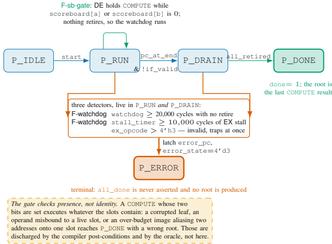
Fig. 12. Property 2. A missing or misrouted operand halts the run; it never silently produces a different root.
