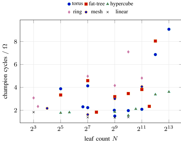
Fig. 20. Distance to the composite lower bound \Omega for every HW-validated instance, against leaf count. A value of 1.0 would mean the compiler achieved the bound exactly; the bound is not known to be tight, so the gap is part slack and part real.
