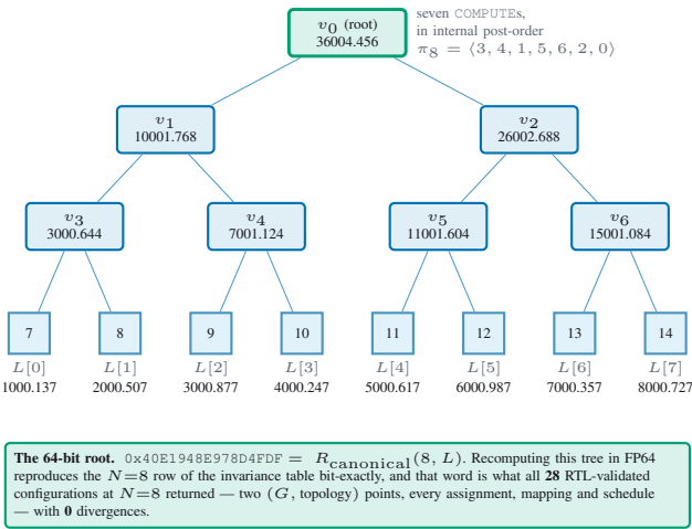
Fig. 5. A worked reduction at N=8 with the real leaf values, reaching the canonical root the campaign reports for that leaf count.
