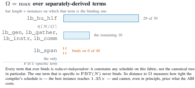
Fig. 16. How \Omega is assembled, and which constituent binds. Every binding term is reducer-independent, which is why distance to \Omega cannot price the ABI.
