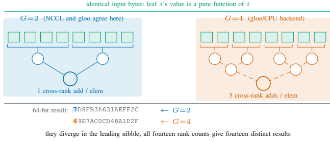
Fig. 2. The premise, measured rather than assumed. Identical bytes reduced at different world sizes yield different 64-bit roots. Above G=2 the sweep runs on the gloo/CPU backend, because NCCL requires one rank per device.
