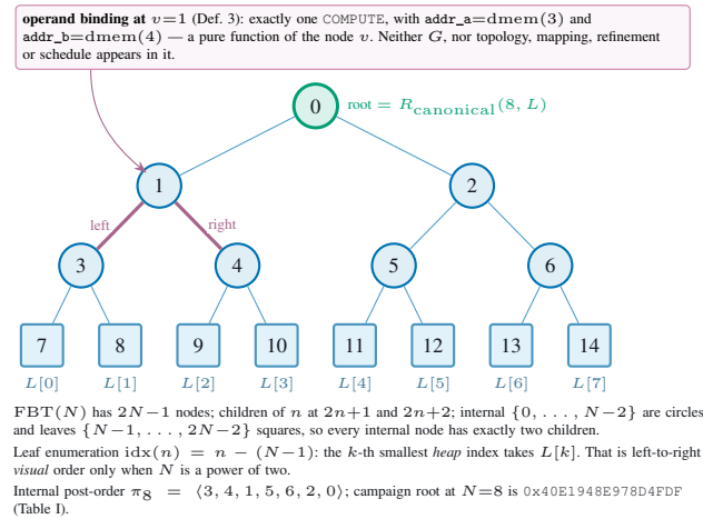
Fig. 3. FBT( N ): heap-indexed, leaves at N-1 \dots 2N-2 ascending. The tree, not the machine, defines the result.
