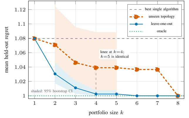
Fig. 21. Held-out regret against portfolio size. The rule transfers to a topology it never saw, and conditioning on topology is worse than ignoring it.
