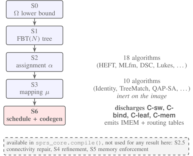
Fig. 15. The compiler pipeline and where each obligation is discharged. Assignment carries the whole decision.
