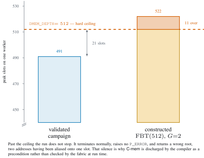
Fig. 13. Peak DMEM occupancy against the hard depth. The campaign came within 21 slots of a ceiling that does not announce itself.
