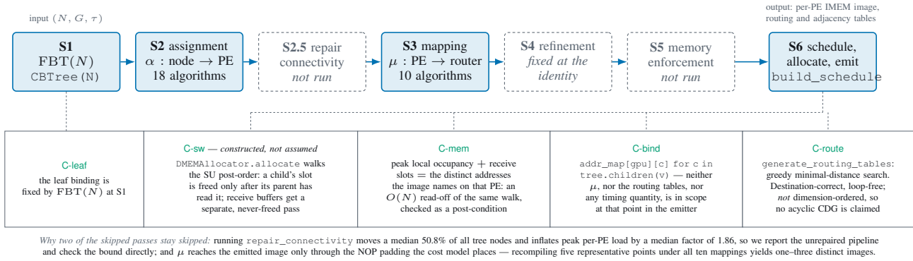
Fig. 15. The compiler pipeline and where each obligation is discharged. Assignment carries the whole decision.
