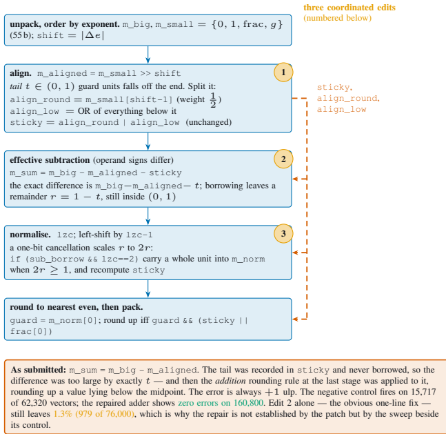
Fig. 2. The effective-subtraction defect and its repair, on the adder datapath. The alignment tail was recorded in sticky but never borrowed from the difference, and the addition rounding rule was then applied to the result. The one thing to take from it is why the fix is three edits and not one: sticky threads every stage, so borrowing the tail changes what the renormalising shift and the final rounding decision mean. Edit 2 alone — the obvious one-line patch — still leaves 1.3% of effective subtractions wrong, which is why correctness here is established by the sweep beside its negative control and not by the patch.
