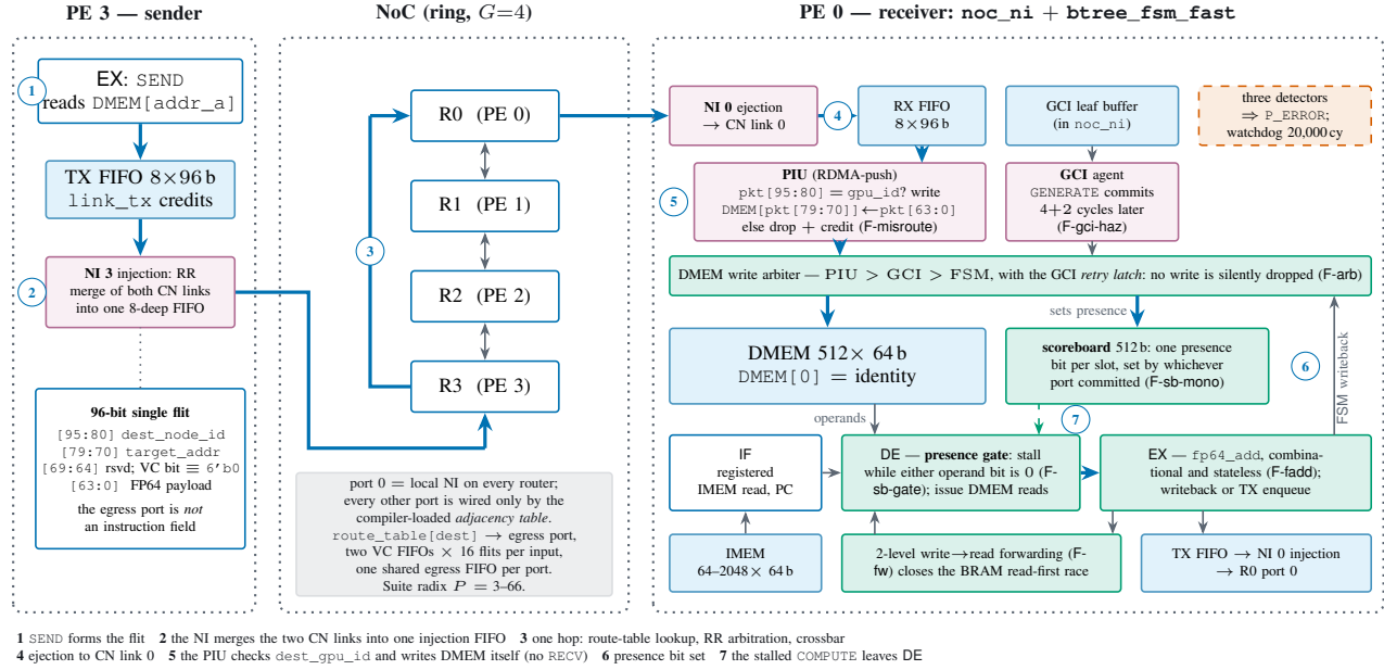
Fig. 1. The fabric, traced along the path one 64-bit operand actually takes: a SEND on PE 3 forms a 96-bit single flit, the network interface merges the two compute-node links into one injection FIFO, the router resolves the egress port from its compiler-loaded route table, and on arrival the PIU — not a RECV instruction, of which there is none — checks dest_gpu_id and writes DMEM itself, dropping and returning credit on a mismatch (F-misroute). The one thing to take from it is the last two steps: the scoreboard is the single source of truth for “data present at address a ” across all three agents that write DMEM (PIU, GCI, FSM writeback), and DE holds the dependent COMPUTE until both operand bits are set, so a scoreboard-gated read is race-free against arrival time. The write arbiter’s GCI retry latch is why no write is silently dropped, and §IV-D shows the latch is necessary for the value , not only for liveness.
