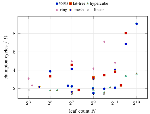
Fig. 3. Distance to the composite lower bound \Omega for every HW-validated instance, against leaf count. A value of 1.0 would mean the compiler achieved the bound exactly; \Omega is assembled from separately-derived constraints and is not claimed tight, so the gap is part slack and part real. The informative reading is additive, not multiplicative — see the text.
