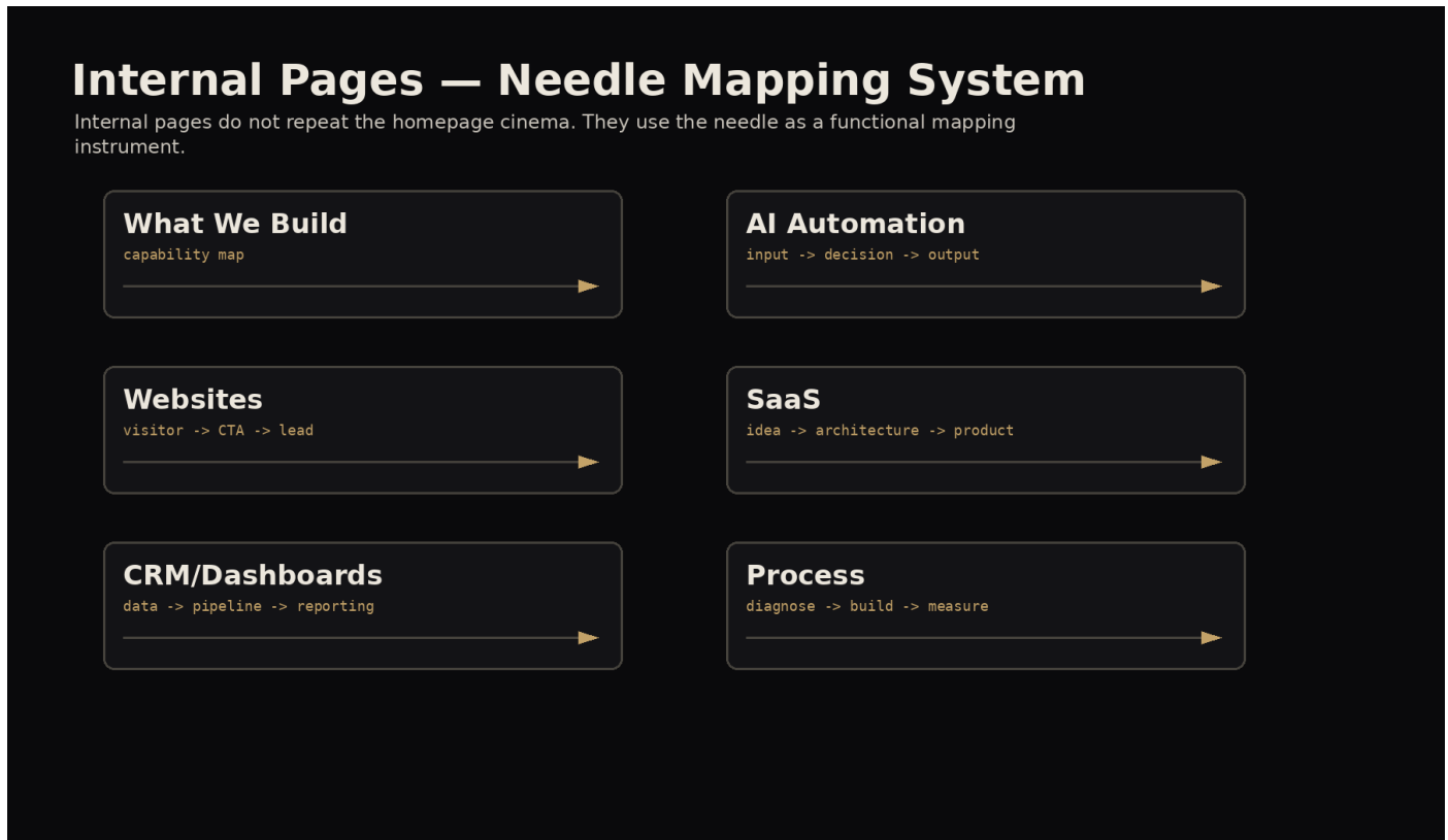
Figure 9: Internal pages
