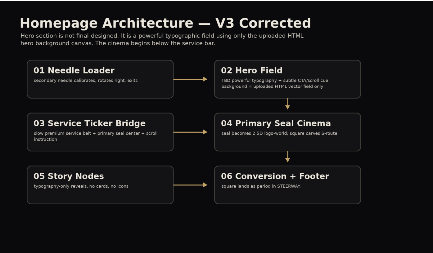
Figure 3: Architecture V3
