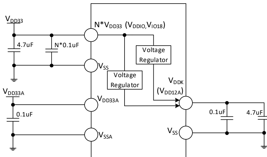
Figure 3-1-6 CH32H416 Conventional power supply typical circuit
