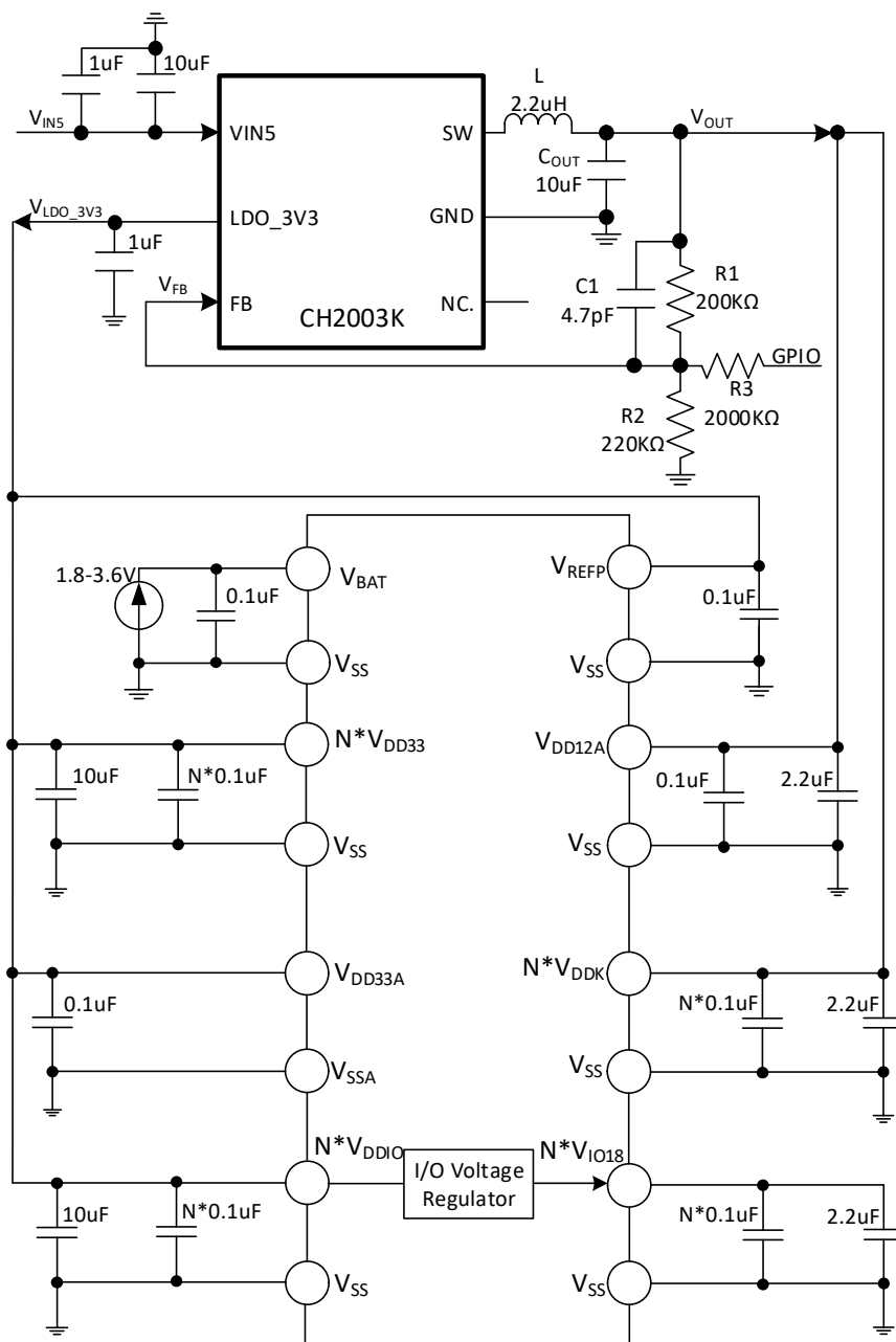
Figure 3-1-3 CH32H417 regulator is a low-power DC-DC single 5V power supply circuit
