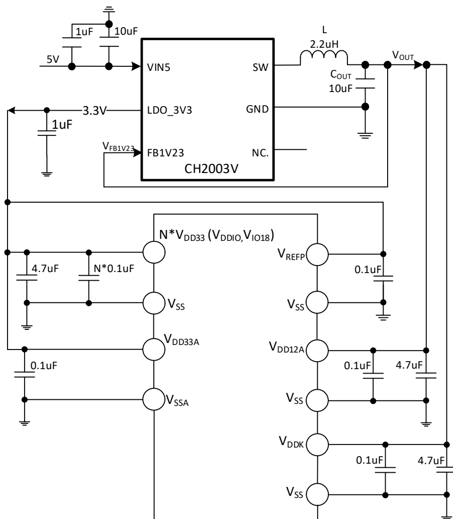
Figure 3-1-5 CH32H416 DCDC single 5V supply circuit
