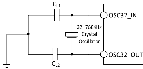
Figure 3-6 Typical Circuit for External 32.768K Crystal
