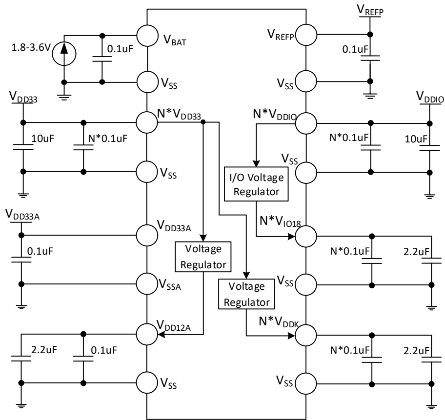
Figure 3-1-1 CH32H417 Conventional power supply typical circuit
