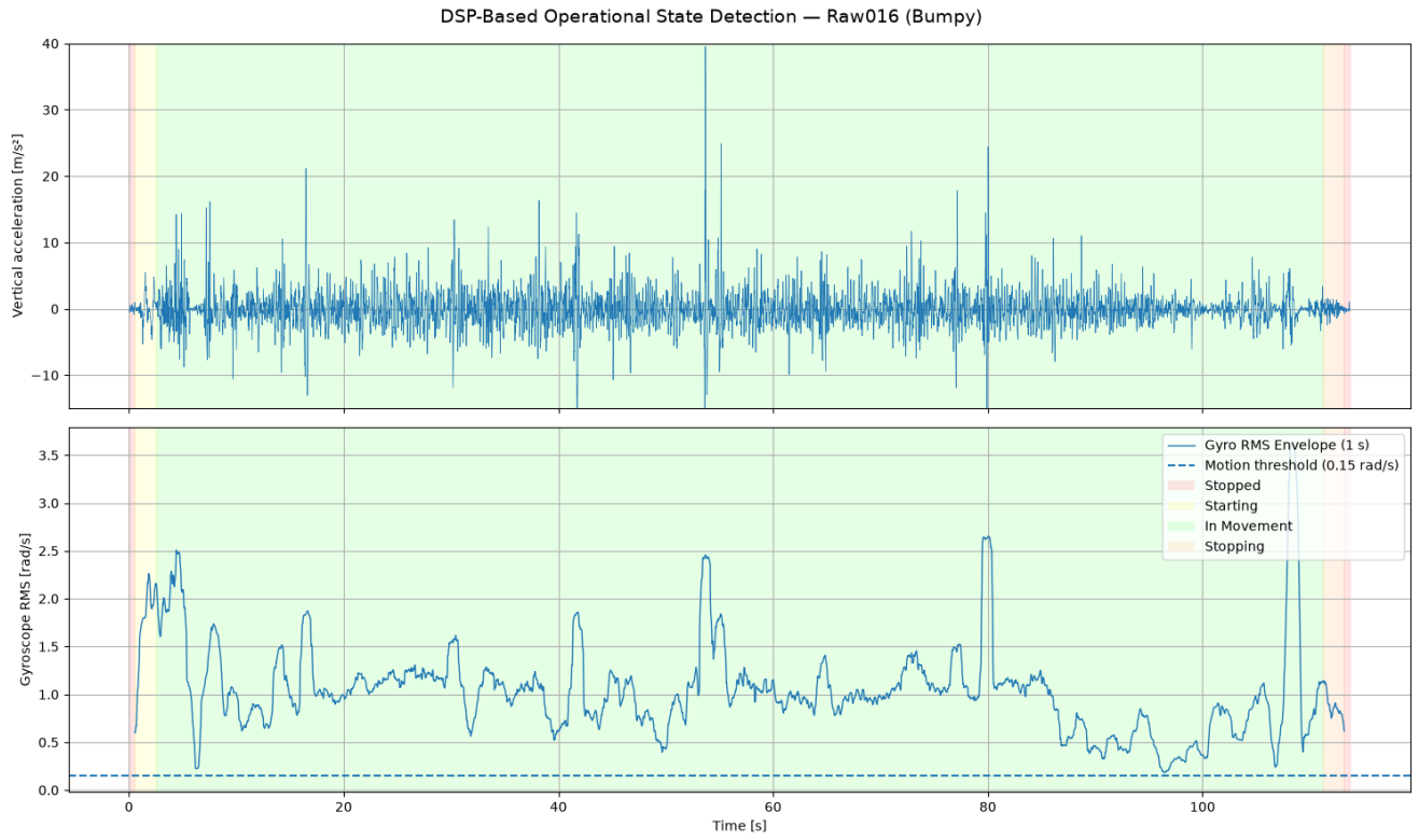
Figure 8: Example of DSP-based operational-state detection for a Bumpy recording. The upper panel shows vertical dynamic acceleration and the lower panel the smoothed gyroscope RMS envelope. Background shading marks samples classified as Stopped, Starting, In Movement and Stopping. Only stable In Movement regions were retained for feature extraction.
