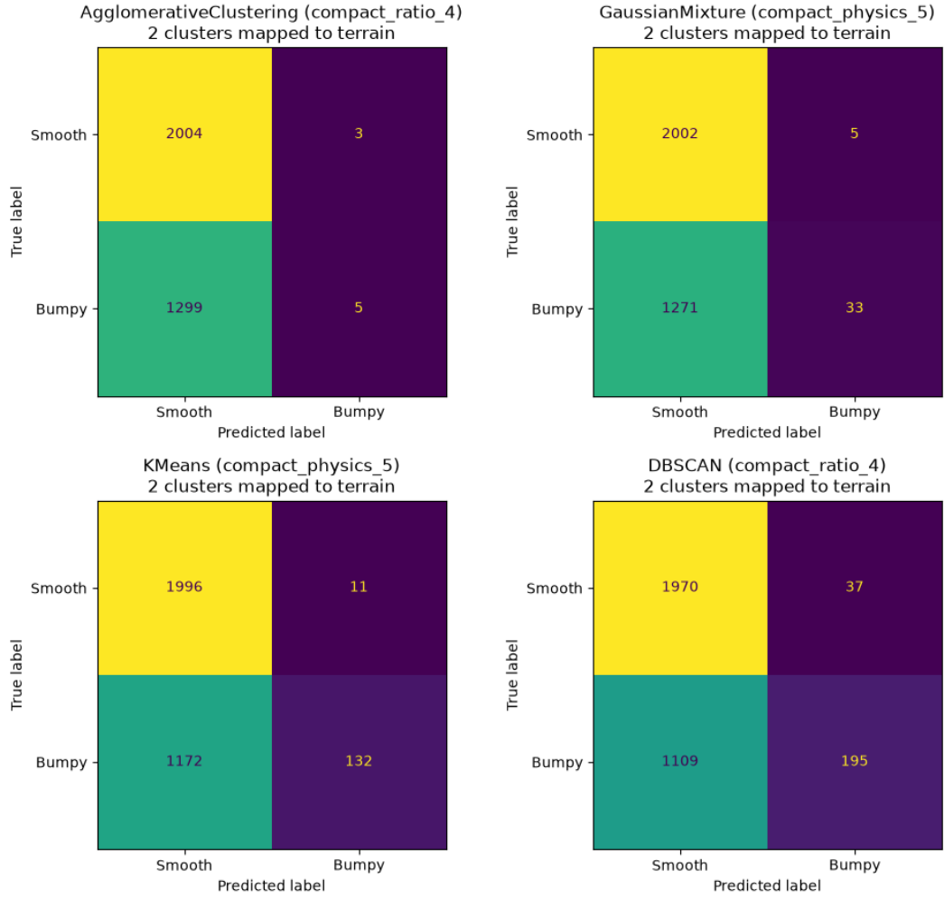
Figure 4: Mapped training-set confusion matrices for the best configuration from each unsupervised clustering family. Terrain labels were not used during clustering and were applied only afterwards to map clusters for diagnostic comparison.
