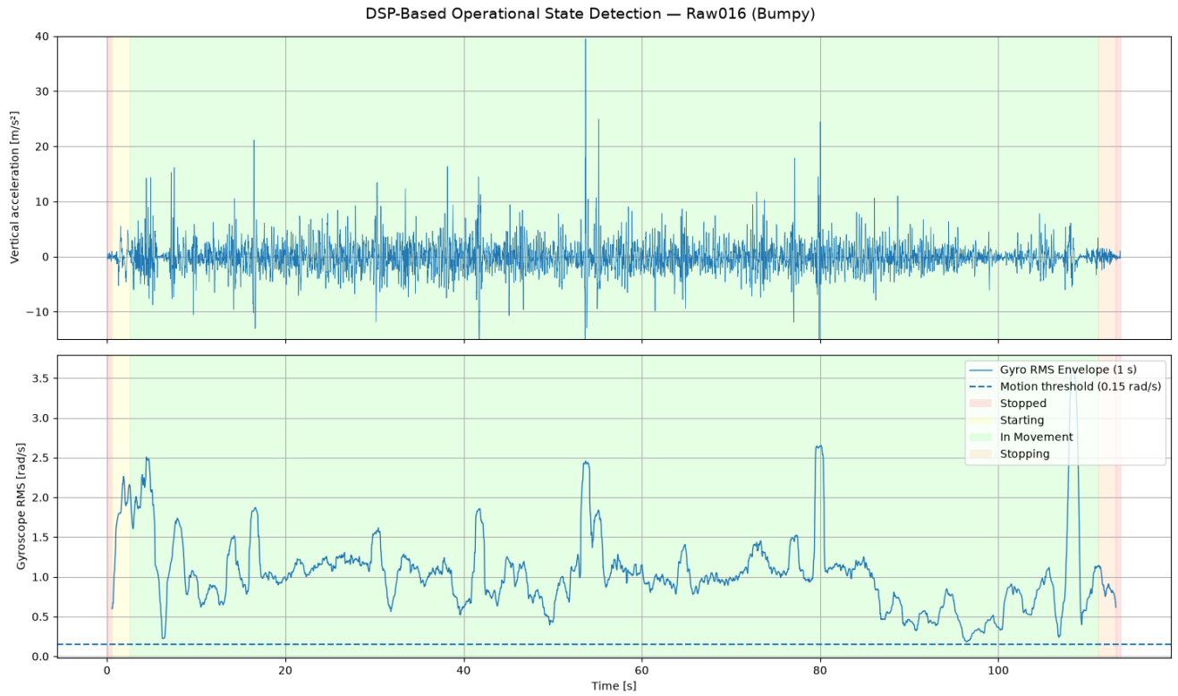
Figure 9: Example of DSP-based operational-state detection for a Bumpy recording. The upper panel shows vertical dynamic acceleration and the lower panel the smoothed gyroscope RMS envelope. Background shading marks samples classified as Stopped, Starting, In Movement and Stopping. Only stable In Movement regions were retained for feature extraction.
