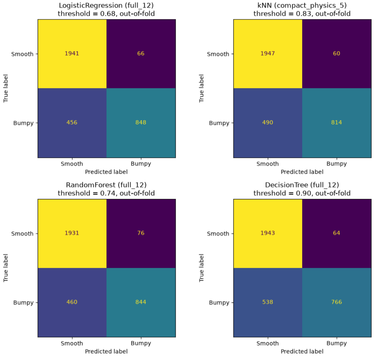
Figure 10: Training-only out-of-fold confusion matrices for the best configuration from each supervised model family. The thresholds shown were selected using out-of-fold training predictions and were fixed before final held-out evaluation. Logistic Regression achieved the highest validation F_{0.5} score and was therefore selected as the final model.
