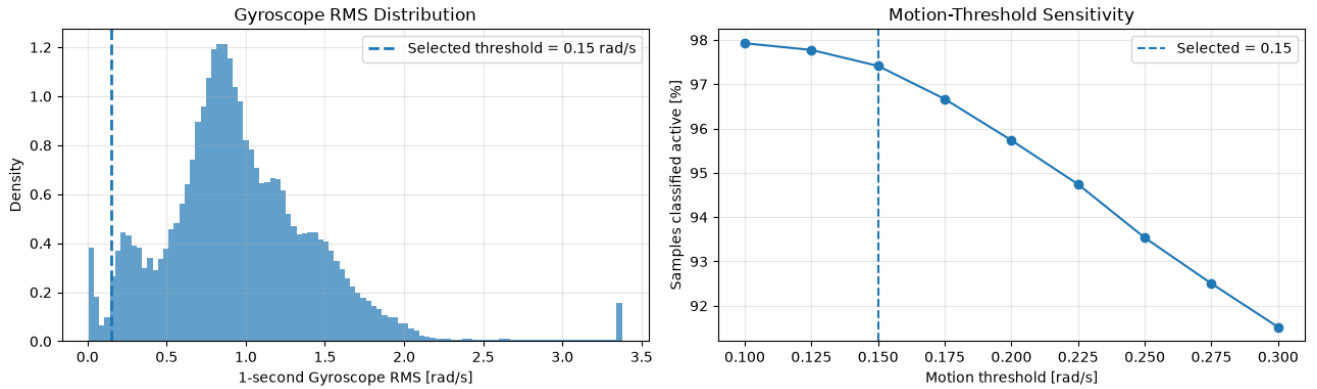
Figure 8: Diagnostic analysis used to select the gyroscope-based motion threshold. The left panel shows the distribution of the one-second gyroscope RMS envelope and the selected threshold of 0.15 rad/s. The right panel shows the sensitivity of the proportion of samples classified as active to alternative threshold values.
