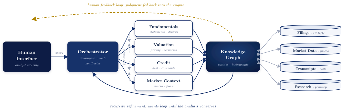
FIGURE 1 · ARCHITECTURE OF THE MULTI-AGENT RESEARCH ENGINE
