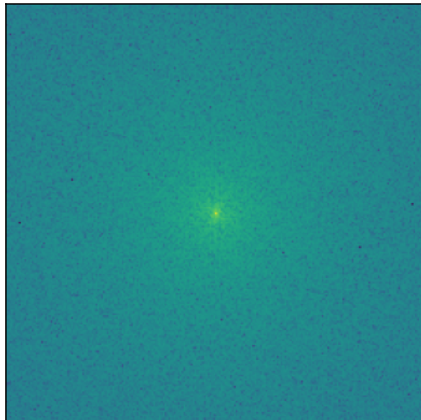
FFT log-magnitude
