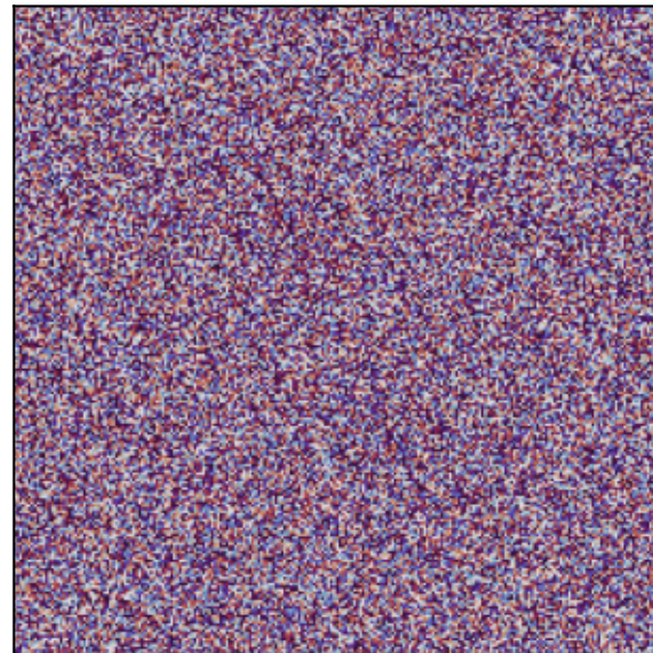
FFT phase
