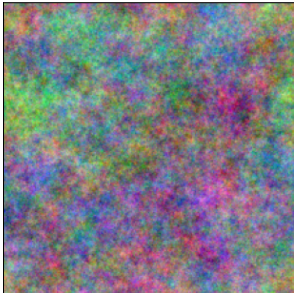
RGB image
