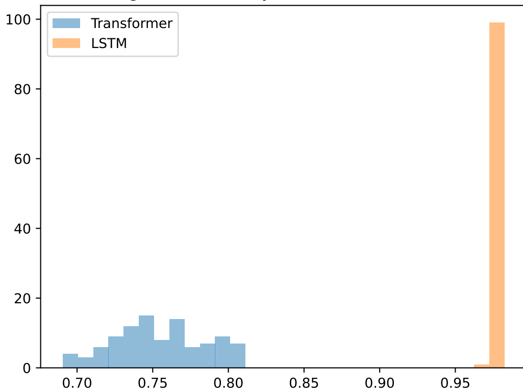
Histogram of accuracy of Transformer and LSTM
