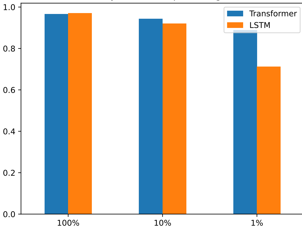
Model accuracy for various percentages of dataset
