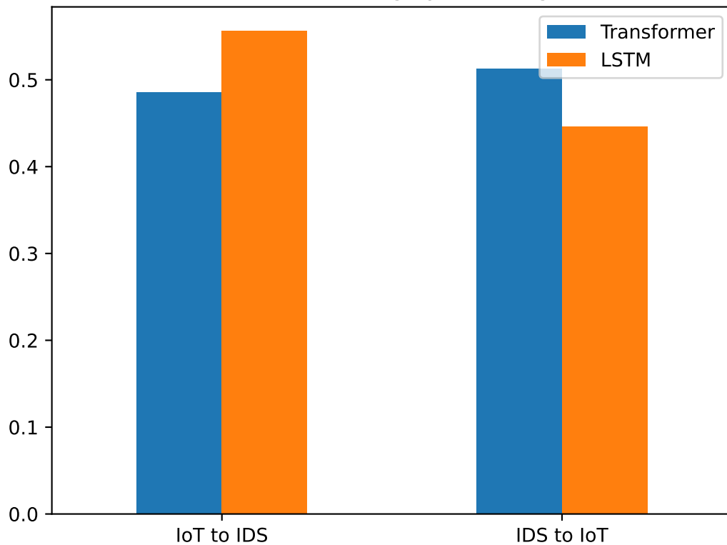
Transfer learning by data origin
