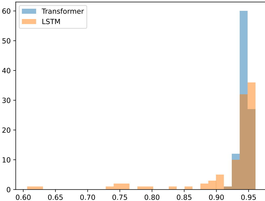
Histogram of F1 score of Transformer and LSTM
