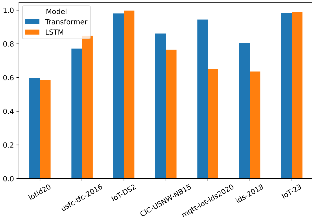
Models accuracy for normal samples
