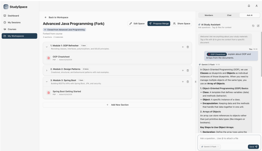
■ Figure 3.15 AI assistant panel: Conversational interface for querying course materials
