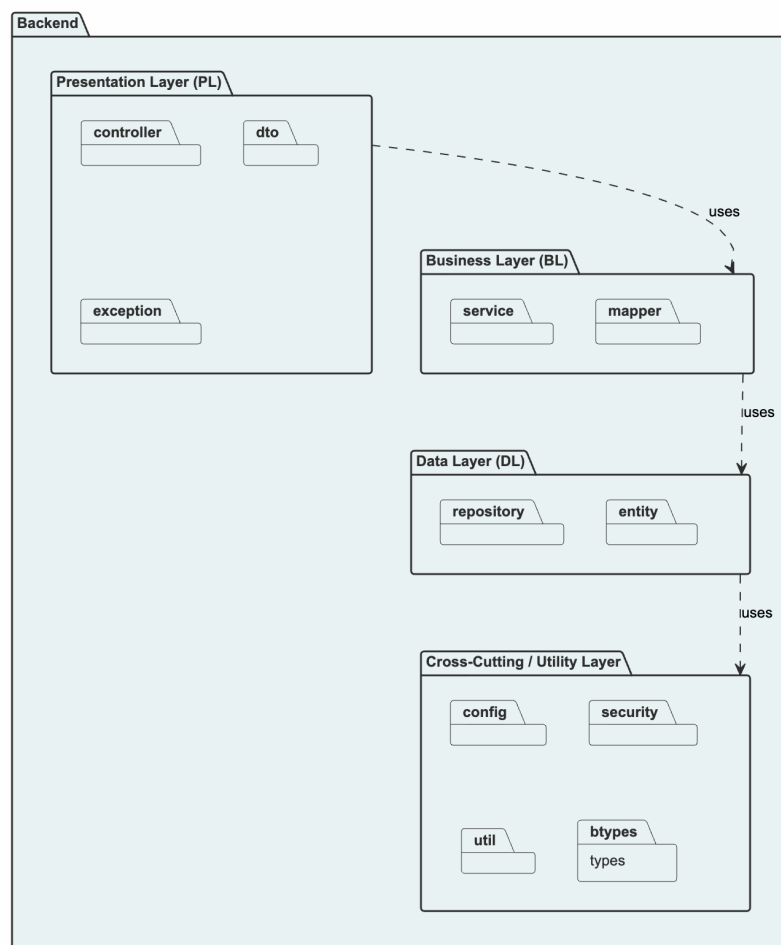
■ Figure 3.5 Logical package architecture of the StudySpace backend
