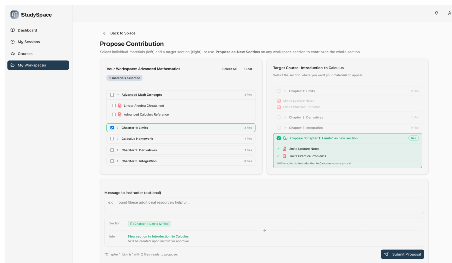
■ Figure 3.13 Merge Proposal submission dialog
