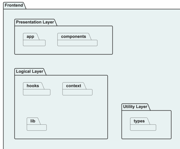
■ Figure 3.6 Logical package architecture of the StudySpace frontend
