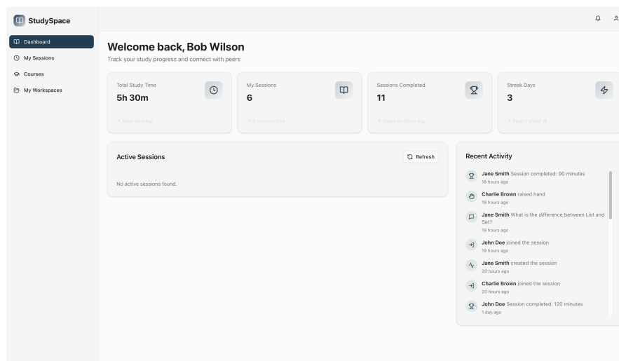
■ Figure 3.10 Student dashboard: The primary entry point featuring recent activities and quick navigation
