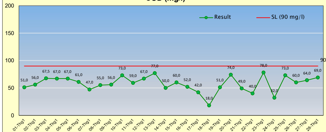
COD (mg/l)
